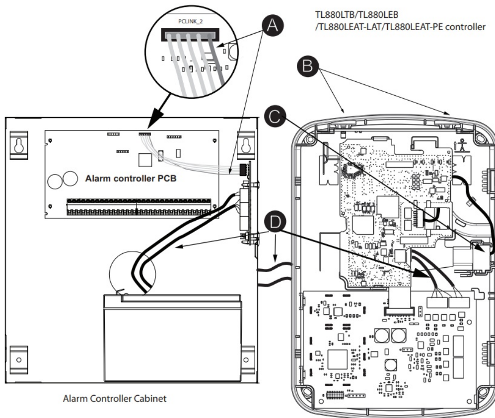
Mounted in Alarm Controller Cabinet
