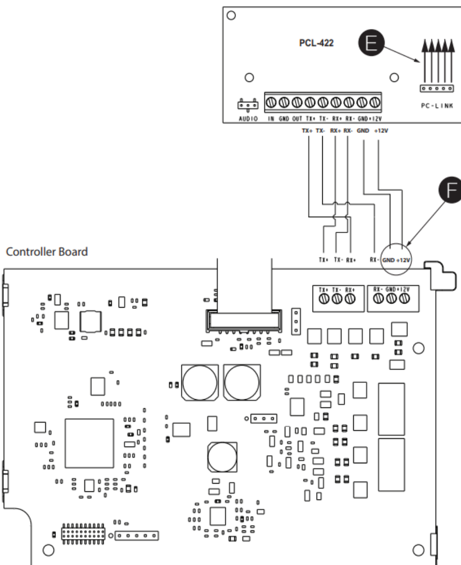
Mounted in Alarm Controller Cabinet
