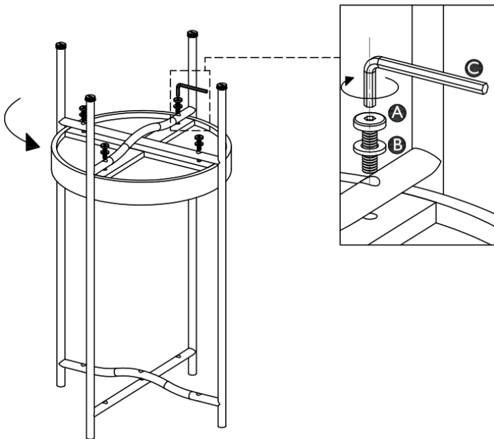
Step 5 Parts, Fittings
