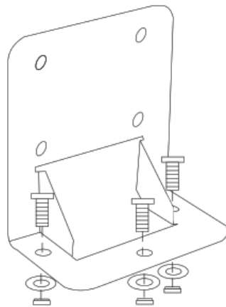
Machine Screws with Nuts (Hole size 7/32")
