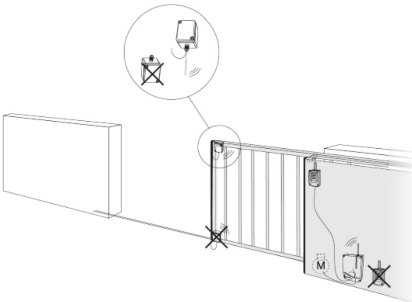
Installation of the Radioband System on a one leaf sliding door with control panel with slot for RADIOBAND/RC-RCS card.
