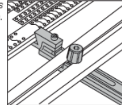
Adjustable slot clamps for PCB fixation.
