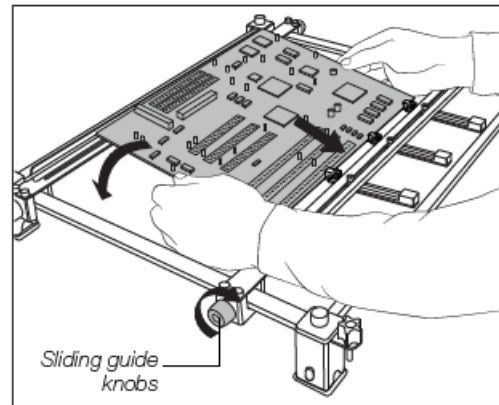
Adjustable slot clamps for PCB fixation.
