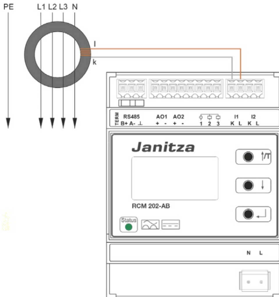
Simplified presentation of residual current measurement
