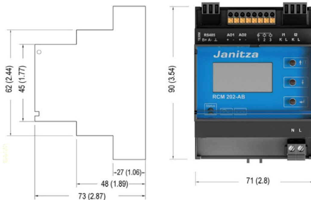
Device dimensions in mm (in)
