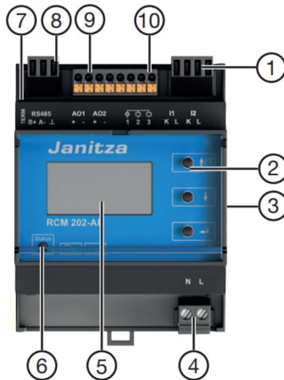
RCM 202-AB device view
