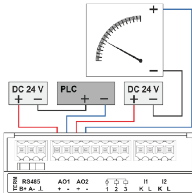
Connection of a display device and a PLC to the analog outputs (Power supply: Janitza power supply unit, art. no. 16.05.012).
