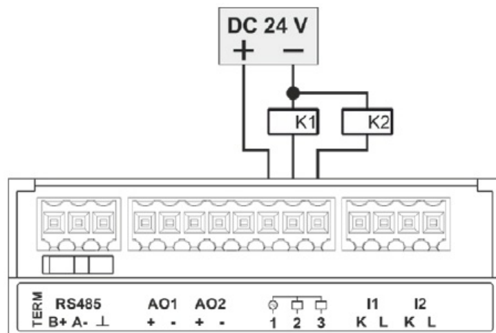
Connection of two relays to the digital outputs
