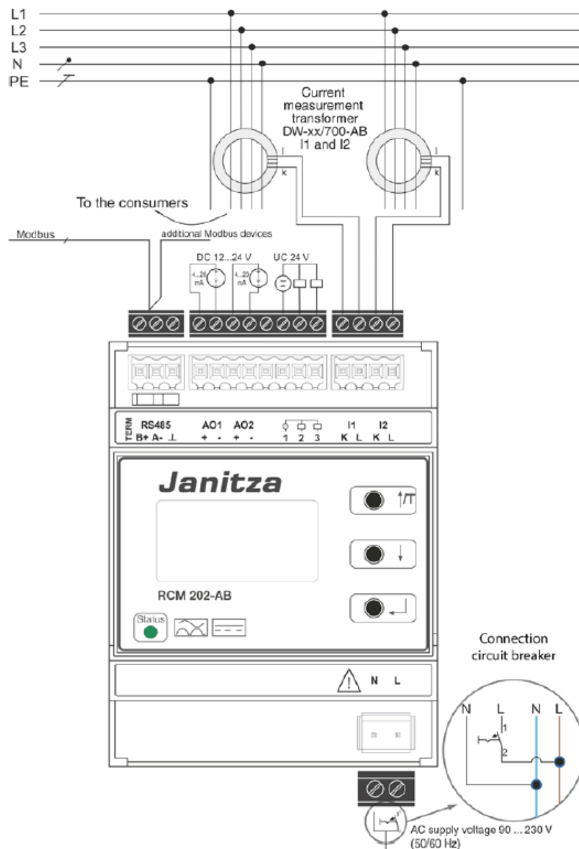
Circuit diagram of the RCM 202-AB
