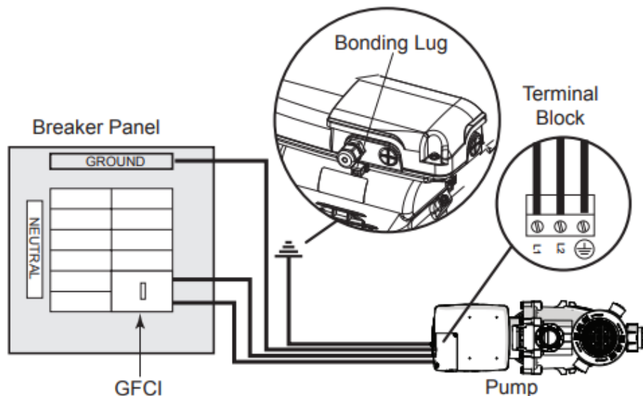
Figure 3. Bonding the Motor
