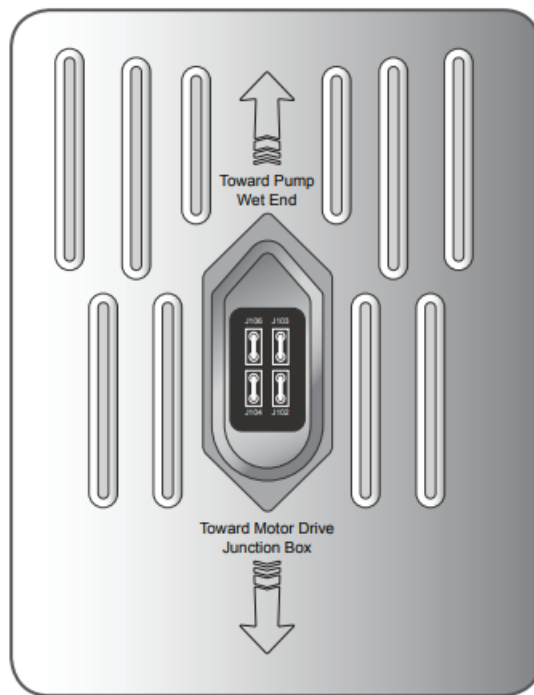
Figure 2. Motor Drive Orientation
