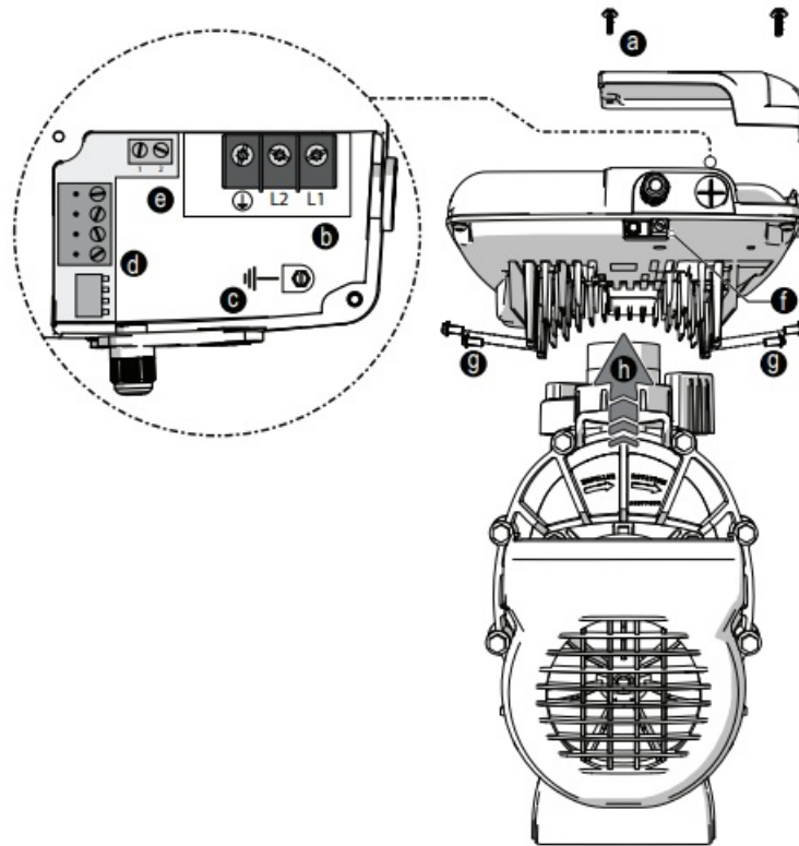
Figure 1. Remove Motor Drive
