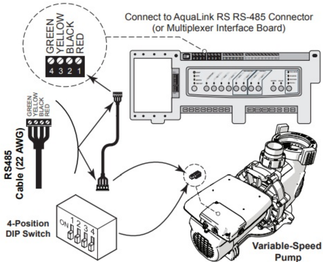
Figure 4. Wiring AquaLink RS, PDA or Z4
