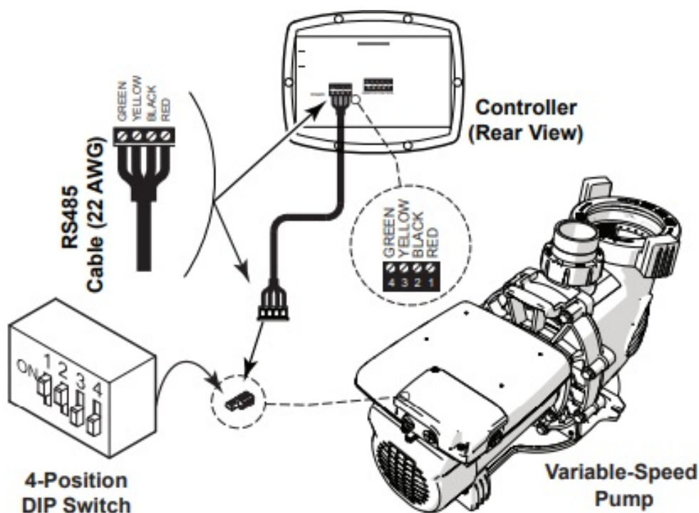
Figure 5. Wiring JEP-R VSP Controller
