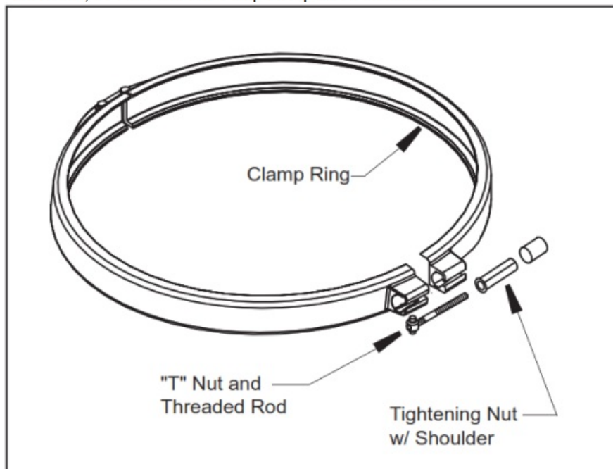
Figure 9. Filter Clamp Ring
