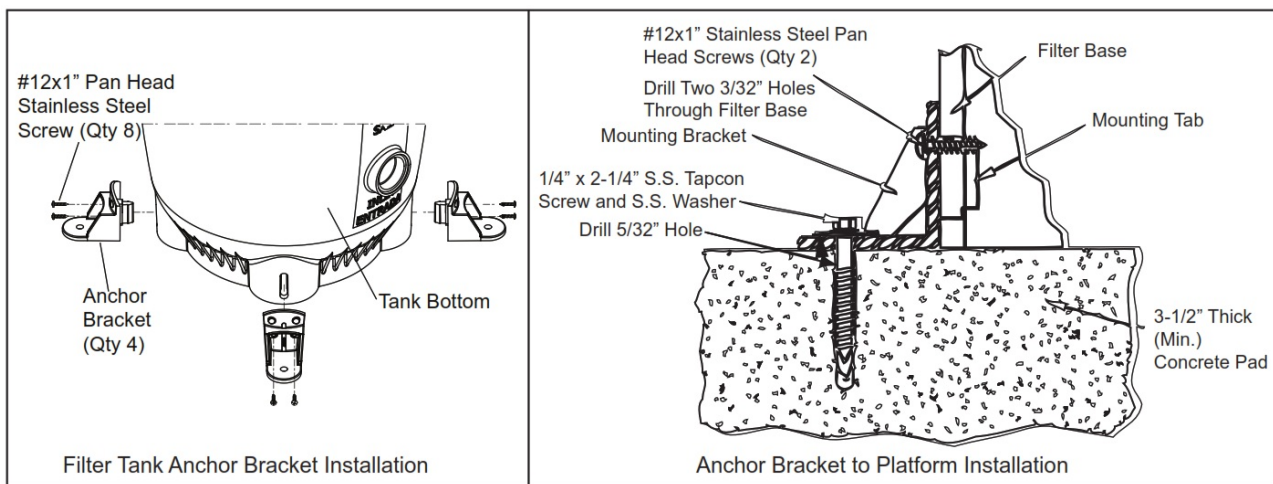
Figure 3. Anchor Bracket Installation
