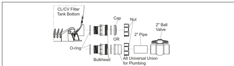
Figure 5A. CV Cartridge Filter Plumbing for Pool/Spa Combination
