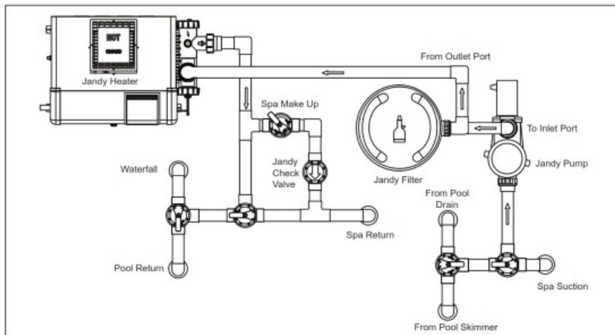
Figure 5. CL Cartridge Filter Plumbing for Pool/Spa Combination
