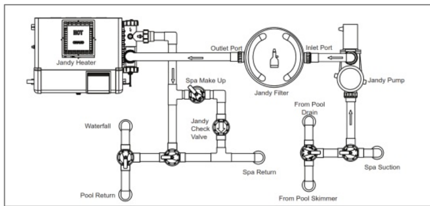
Figure 6. Jandy CL and CV Series Cartridge Filter Drain Configurations
