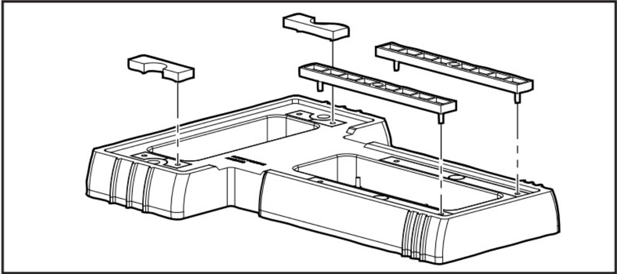
Figure 5. Snap Spacers into Place
