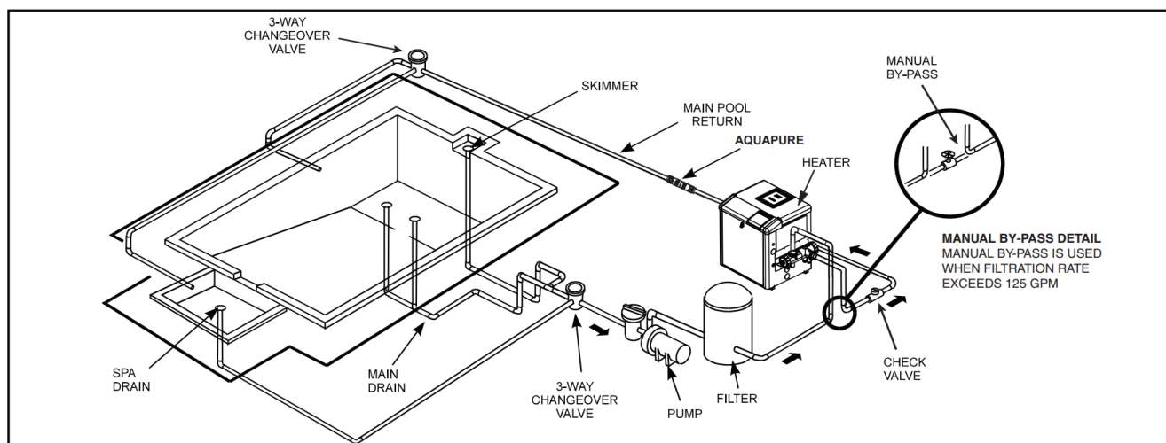
Figure 2. Typical Piping Installation
