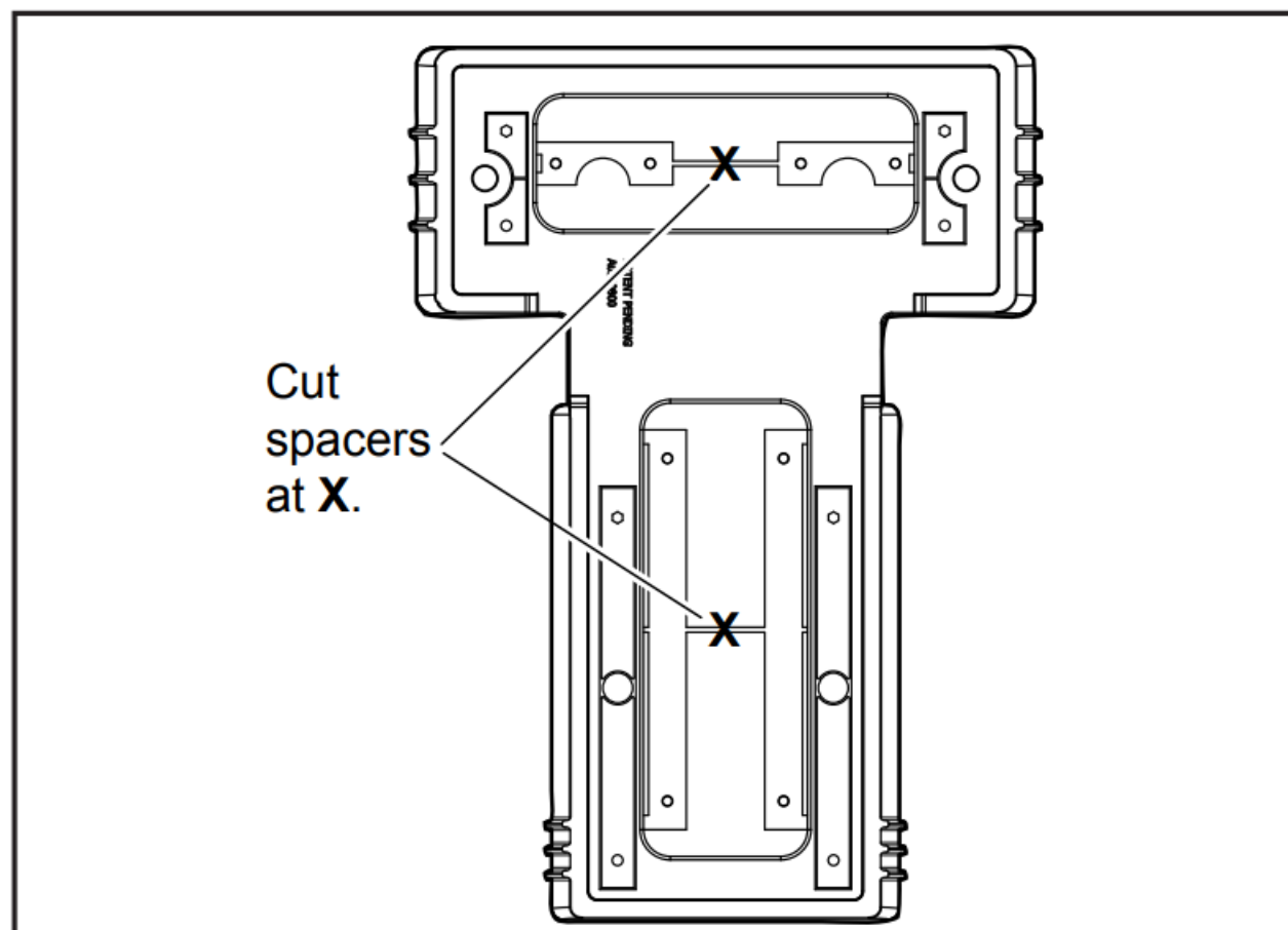
Figure 4. Cut Sets of Spacers Out of Base
