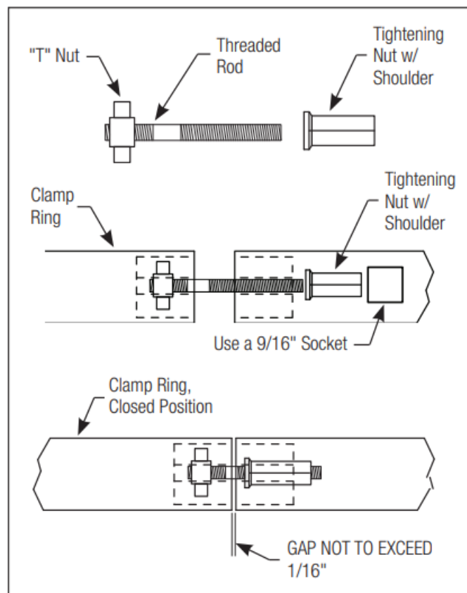
Figure 10. Filter Clamp Ring Assembly
