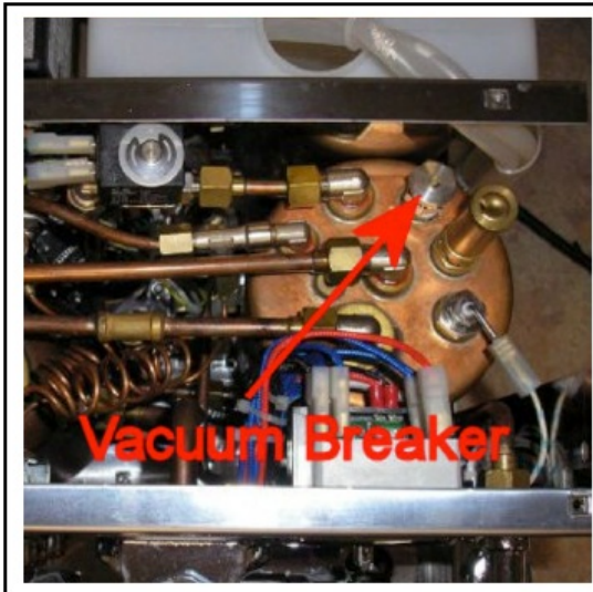
Old Style Vacuum Breaker
