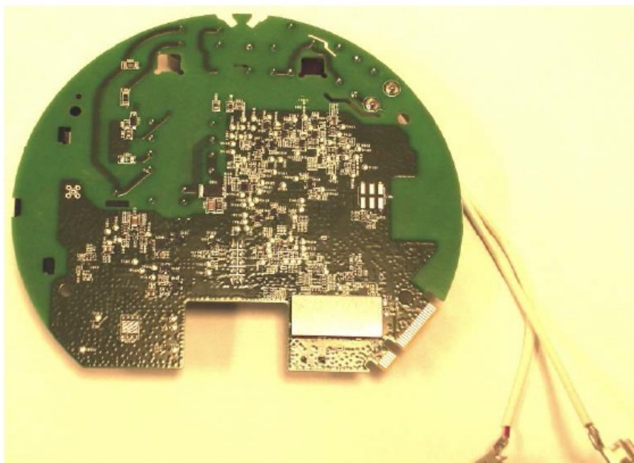
Meter Base (showing metrology)
