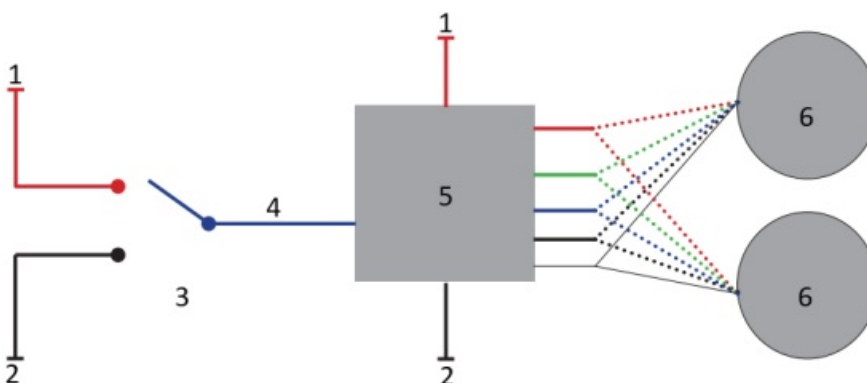
THREE-WIRE SWITCH CONTROL
