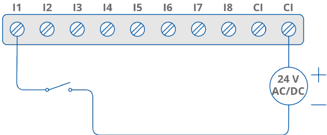
Figure 8. Connection of input
