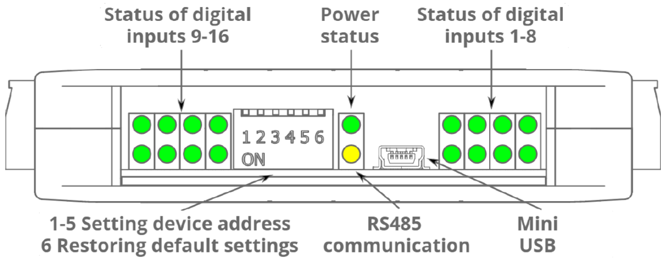
Figure 2. Indicators
