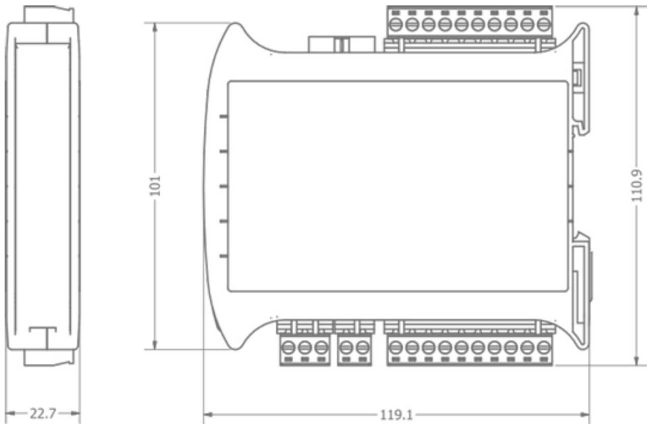
Figure 1. Dimensions
