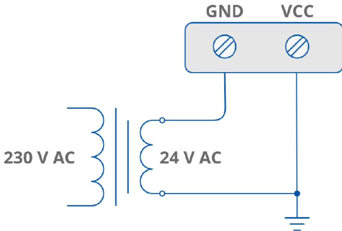
Figure 5. AC power connection
