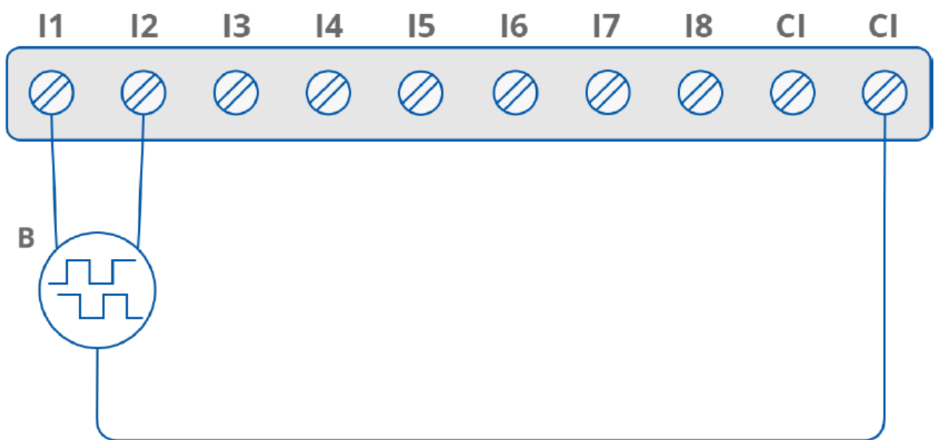
Figure 7. Connection of encoder
