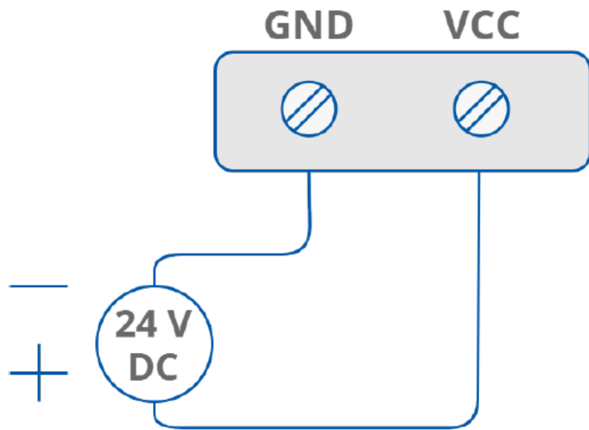
Figure 4. DC power connection
