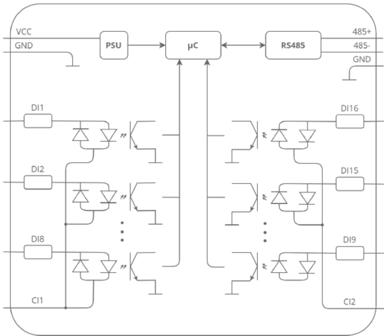
Figure 3. Block diagram
