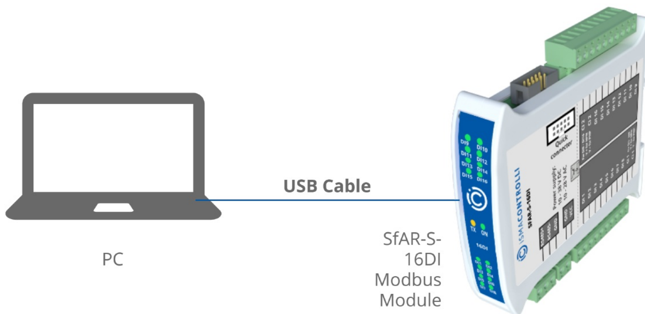
Figure 11. PC connection
