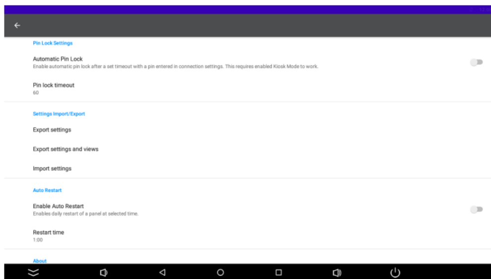
Figure 20. Settings
