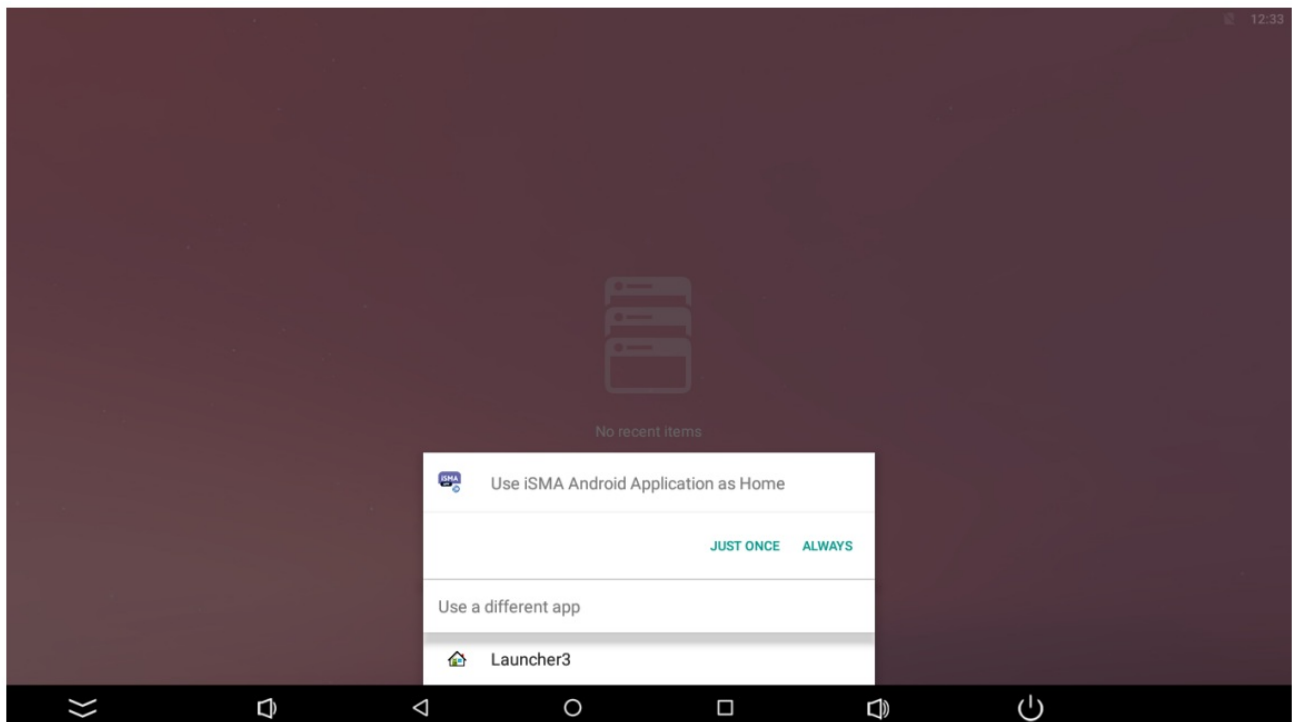
Figure 9. Home application
