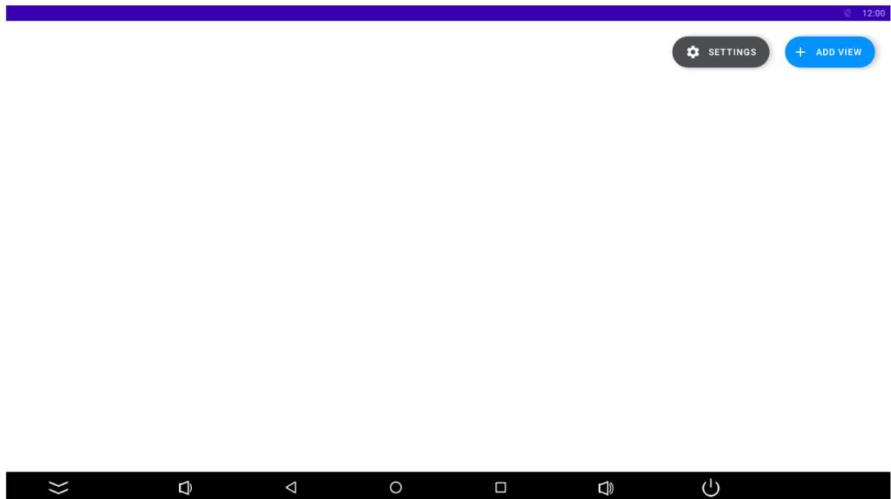
Figure 10. Main screen
