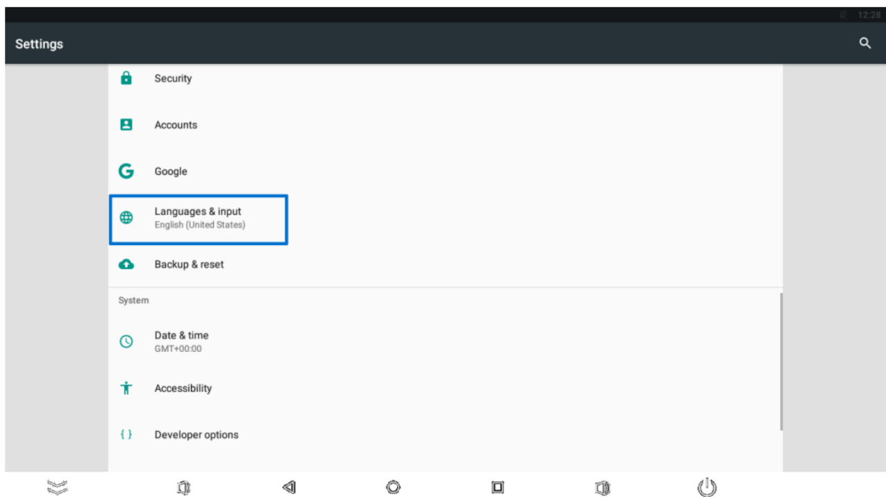
Figure 26. Language settings
