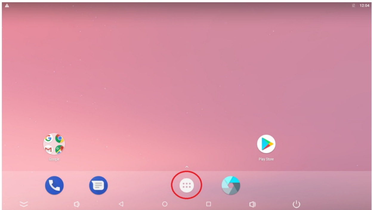
Figure 24. Main screen
