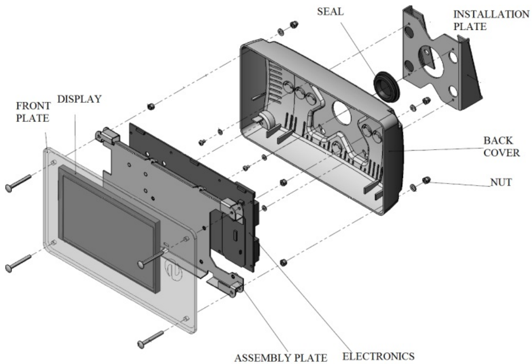
Picture 1 Exploded view
