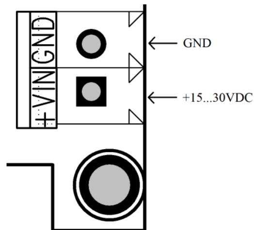
Picture 7 Power connection
