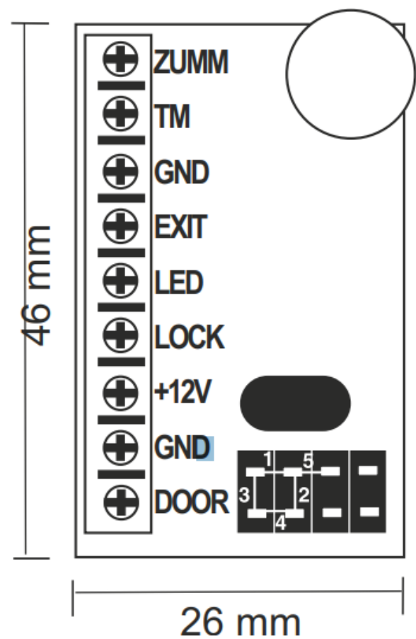
Figure 2: Controller PCB layout
