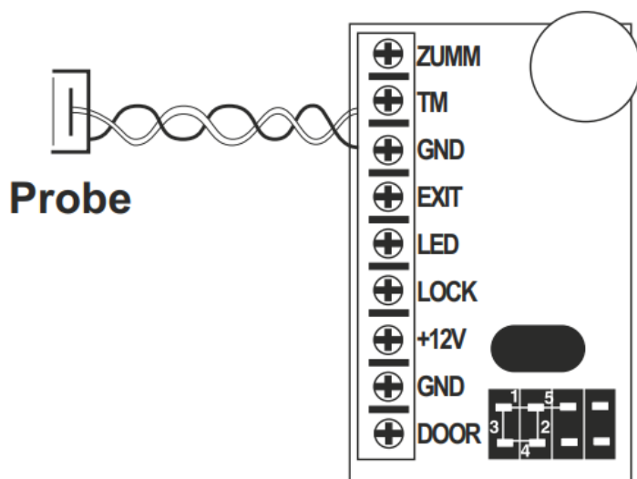
Figure 6. Connecting external devices.
