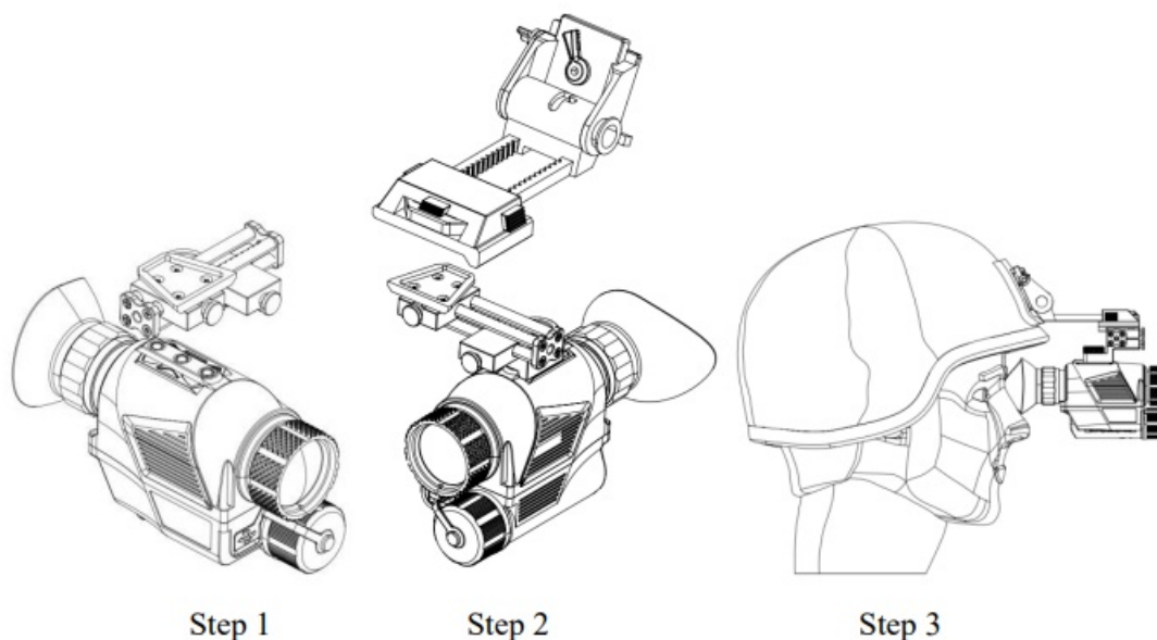
Figure 2.2 J-YM2.0 Installation Diagram for Helmet-mounted Use
