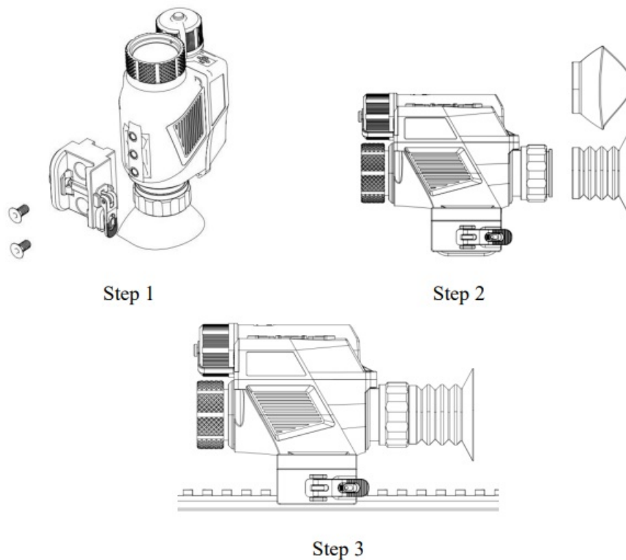
Figure 2.3 J-YM2.0 Thermal Scope Installation Diagram
