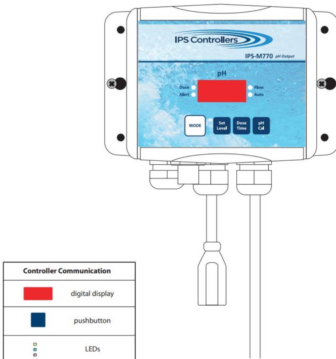
Figure 2: M770 Controller Components Connections
