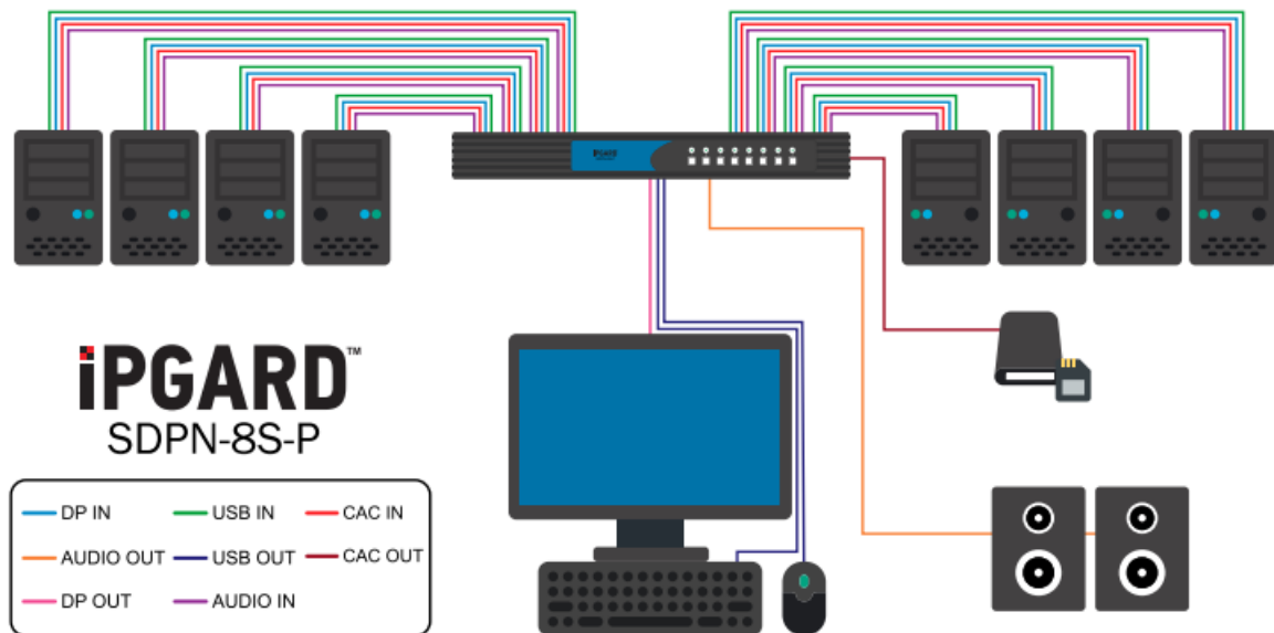
Figure 8-1: SDPN-8S-P
