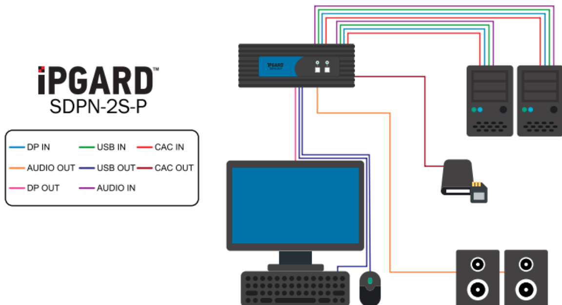
Figure 8-2: SDPN-2S-P
