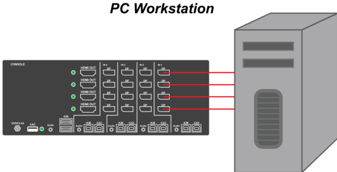
Figure 7-1: SDPN-4Q-P
