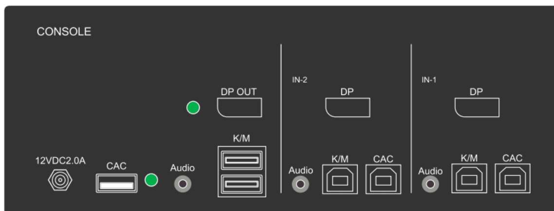
Figure 4-2: SDPN-2S-P Rear panel
