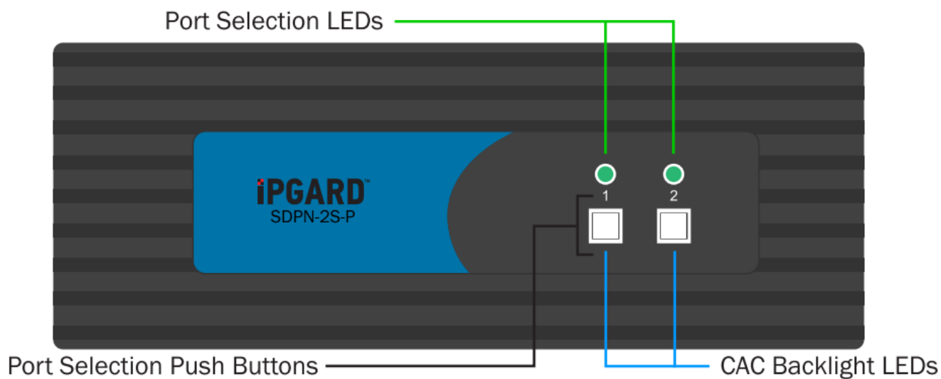
Figure 4-1: SDPN-2S-P Front panel
