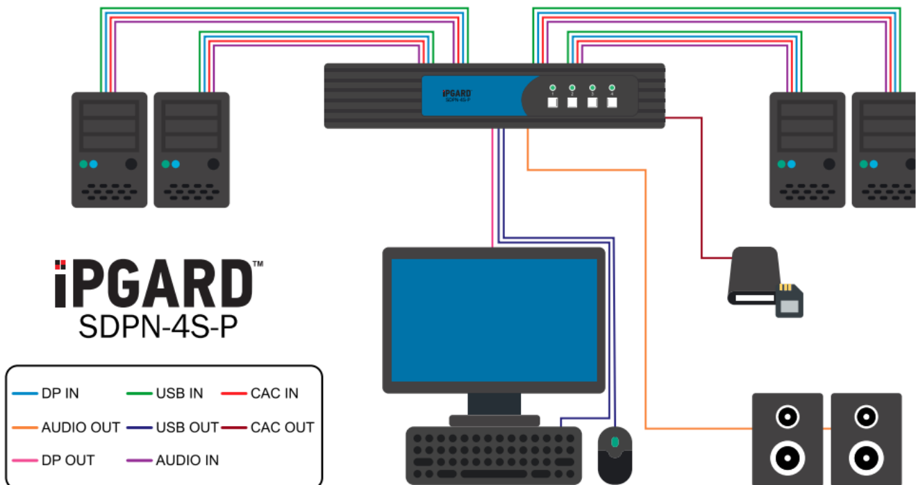
Figure 6-1: SDPN-4S-P
