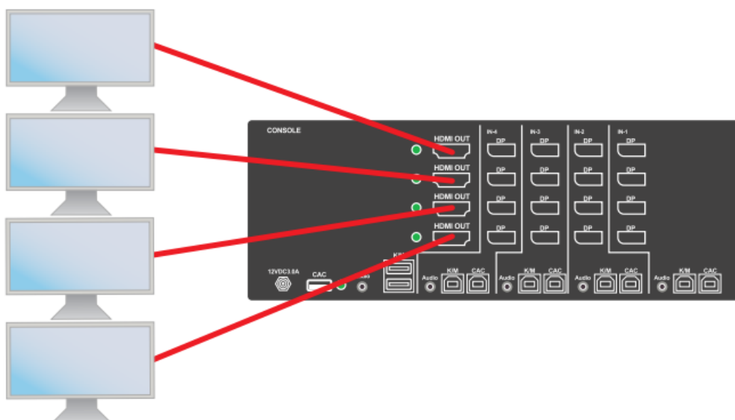
Figure 7-2: SDPN-4Q-P
