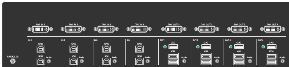
Figure 5-2: SDVN-44-X Rear panel
