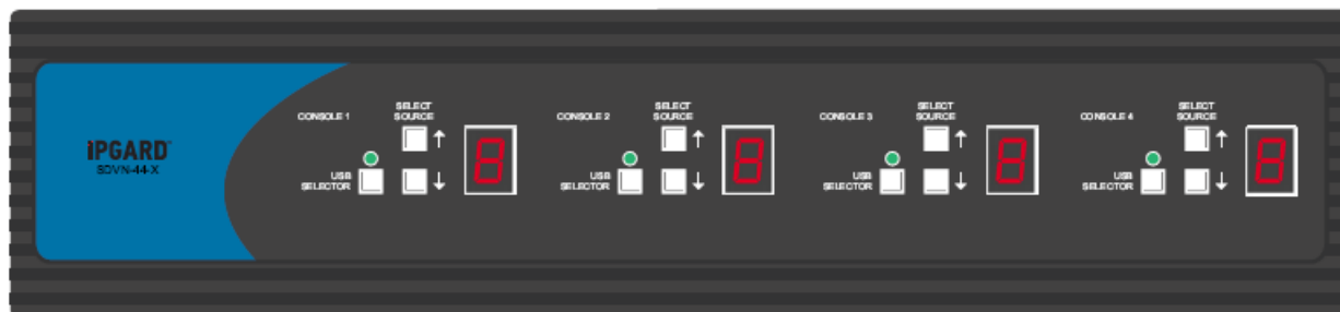
Figure 5-1: SDVN-44-X Front panel
