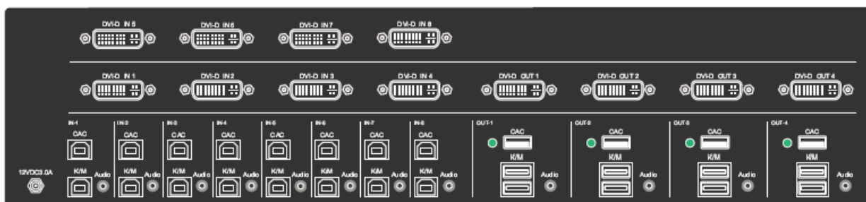
Figure 5-6: SDVN-84-X Rear panel
