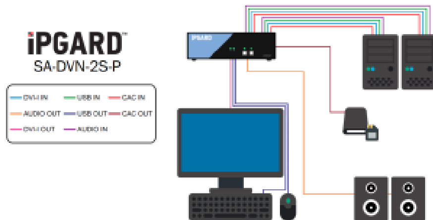
Figure 8-2: SA-DVN-2S-P
