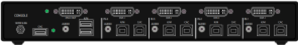
Figure 4-2: SA-DVN-4S-P Rear panel
