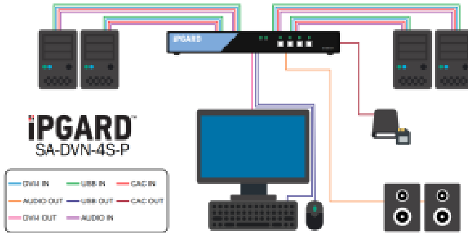
Figure 6-1: SA-DVN-4S-P
