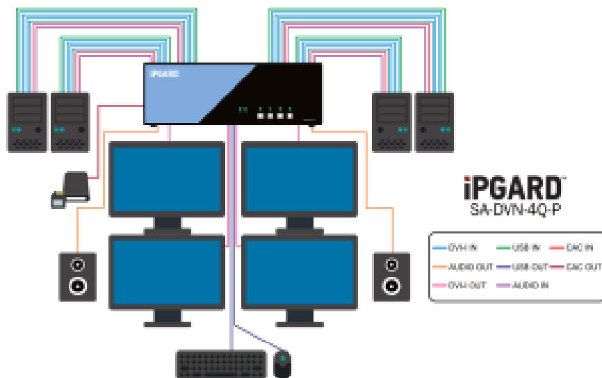
Figure 8-1: SA-DVN-4Q-P
