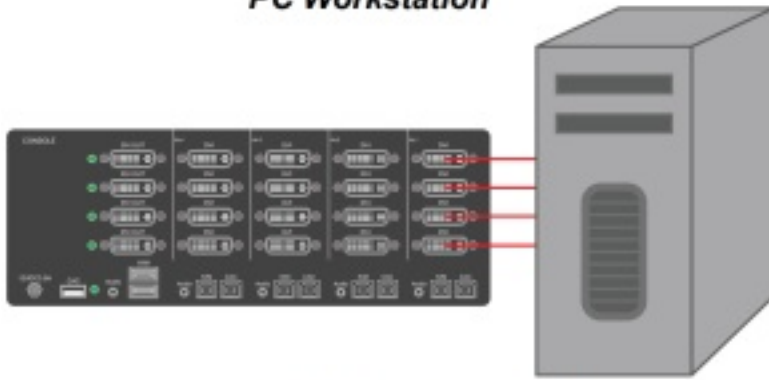
Figure 7-1: SA-DVN-4Q-P
