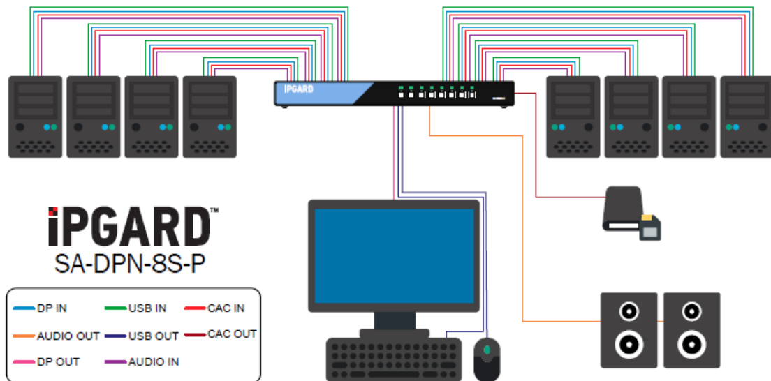
Figure 8-1: SA-DPN-8S-P
