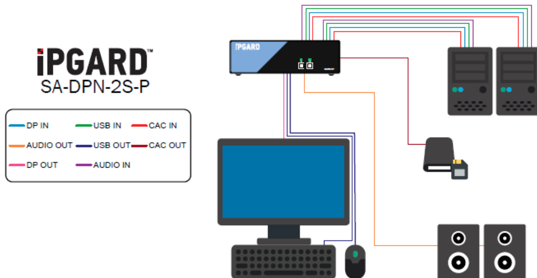
Figure 8-2: SA-DPN-2S-P
