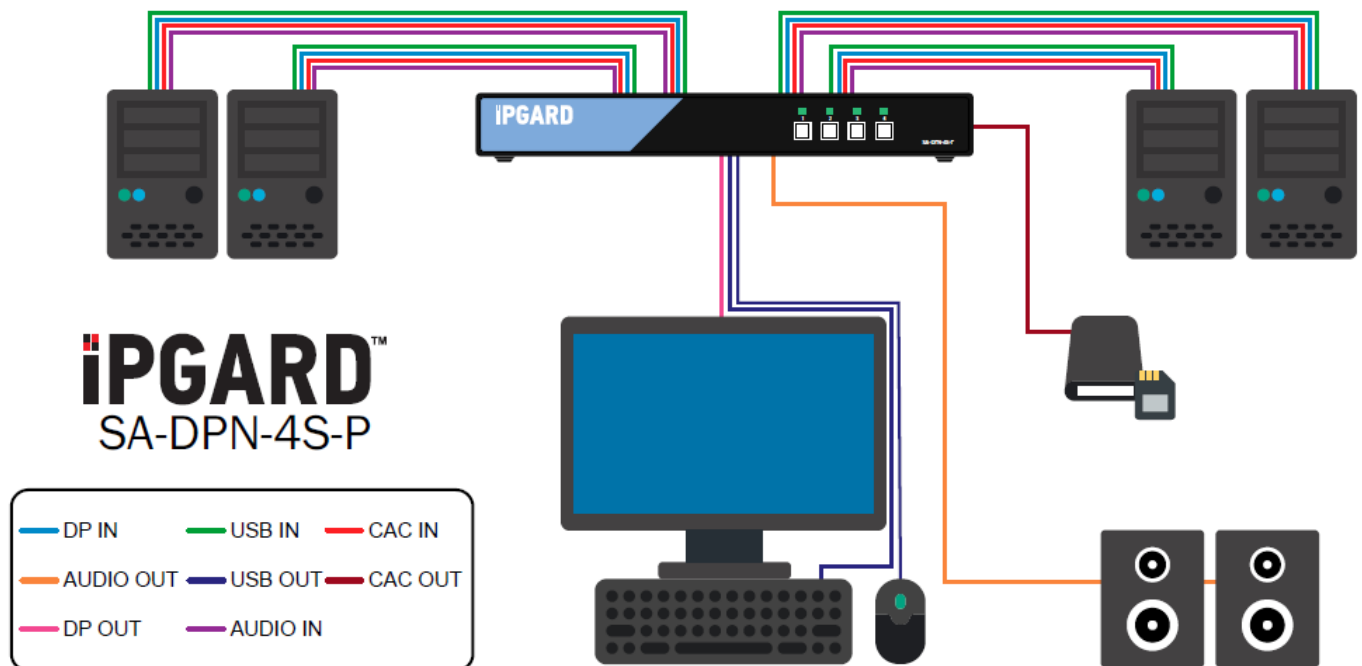
Figure 6-1: SA-DPN-4S-P
