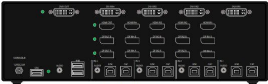
Figure 4-2: SA-DPH-4Q-P Rear panel
