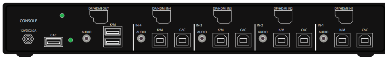
Figure 4-2: SA-HDN-4S-P Rear panel
