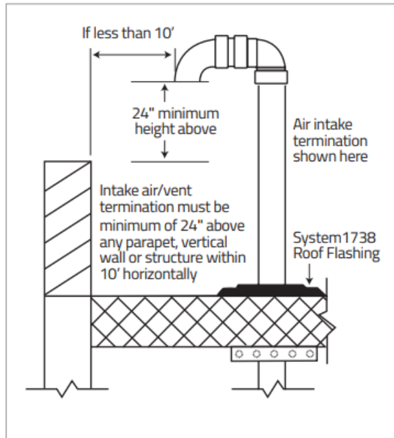
Figure 10: Flat Roof Snorkel Termination
