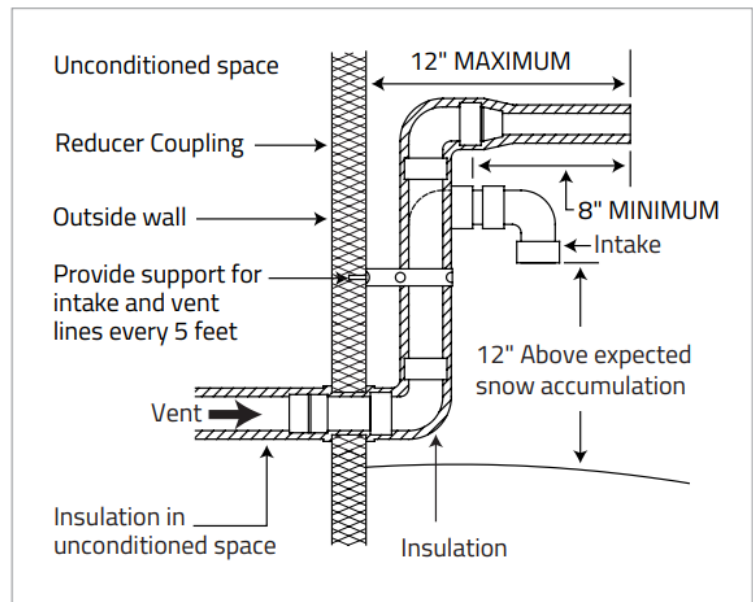
Figure 4 Side View: Typical Wall Snorkel Termination
