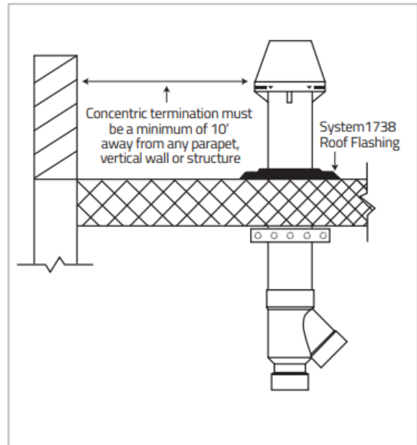
Figure 11: Concentric Vent Flat Roof Snorkel Termination
