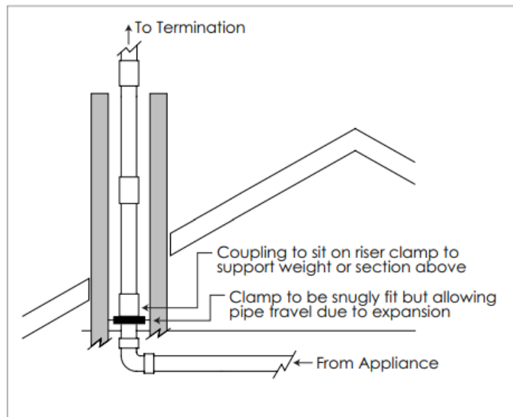
Figure 12: Chimney Termination
