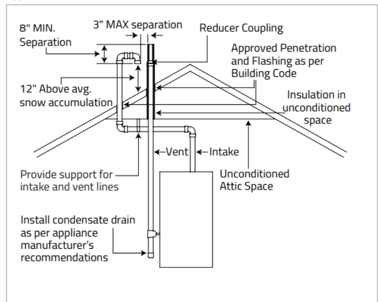
Figure 2 Typical Roof Snorkel Termination
