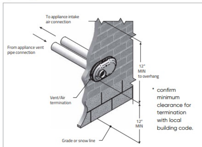
Figure 6: Typical Low Profile Termination
