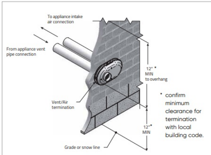
Figure 13: Typical Side Wall Termination
