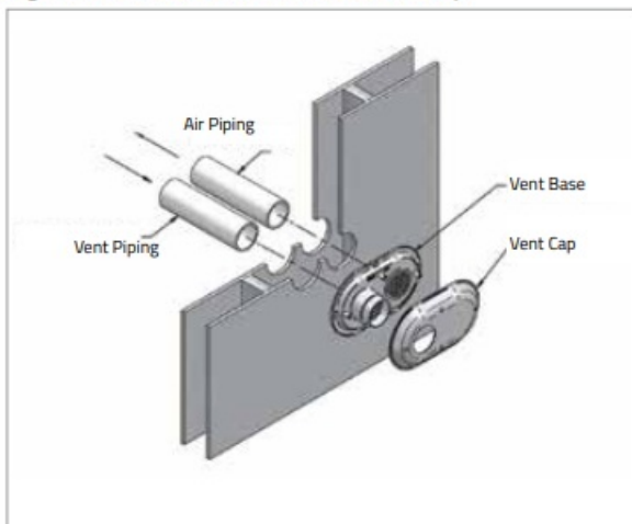
Figure 15: Sidewall Termination Assembly
