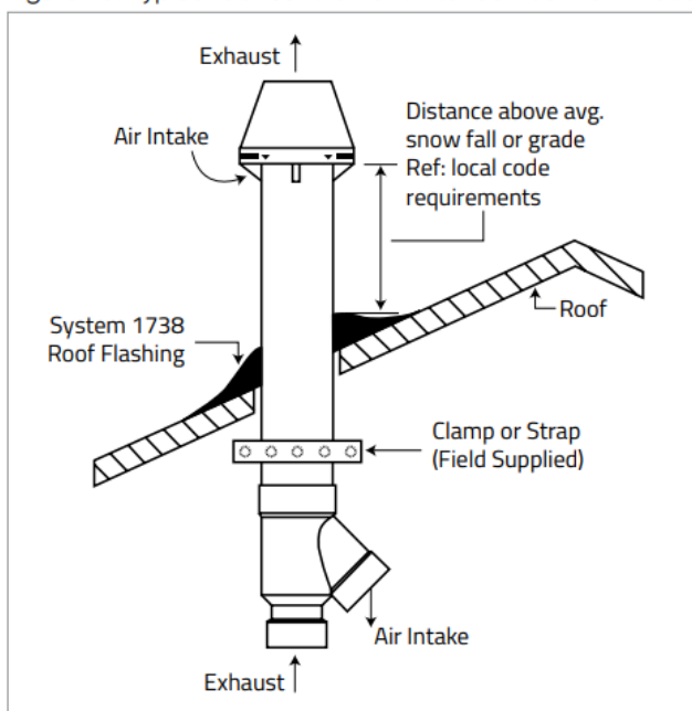
Figure 20: Typical Concentric Vent Pitched Roof Termination
