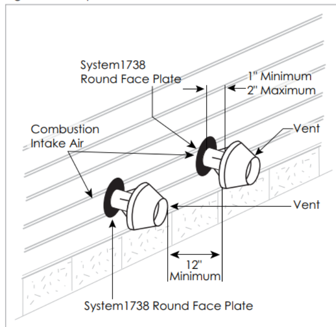
Figure 22: Multiple Concentric Vent Terminations: HORIZONTAL
