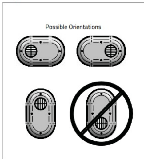
Figure 5: Low Profile Termination - Approved Installation Orientation
