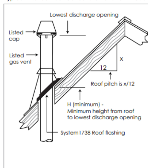
Figure 9: Typical Pitched Roof Concentric Vent Termination
