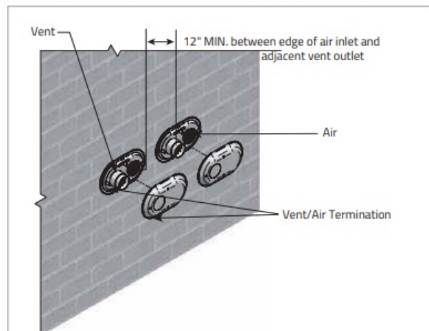
Figure 16: Minimum Clearances: Multiple Side Wall Terminations
