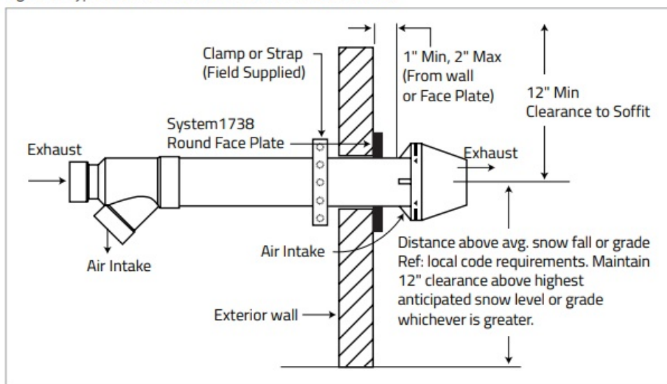
Figure 7: Typical Concentric Vent Side Wall Termination
