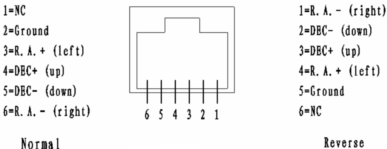
Figure 17. ST-4 guiding port wiring direction
