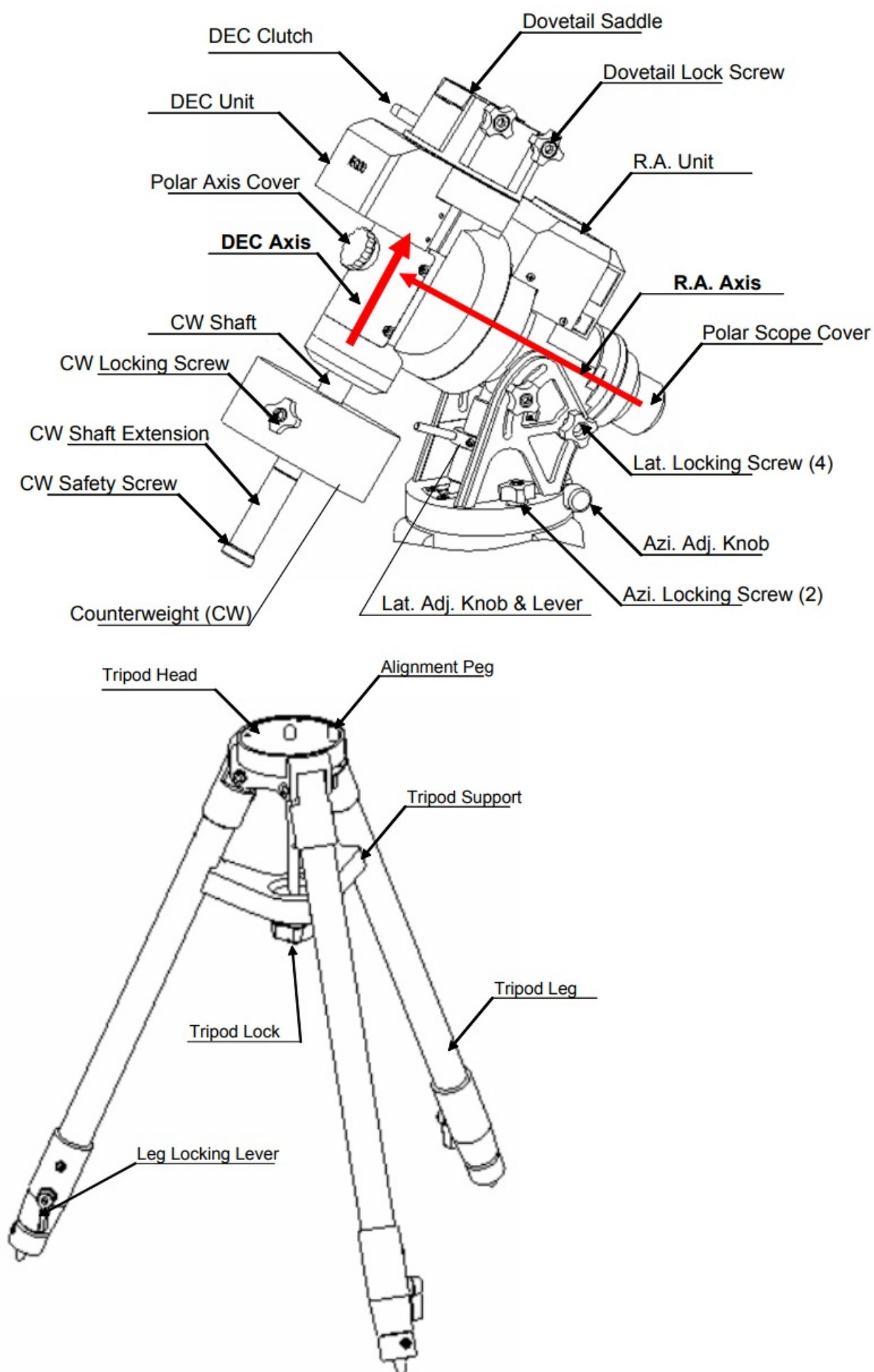
Figure 1. iEQ30 assembly terms (mount and tripod)
