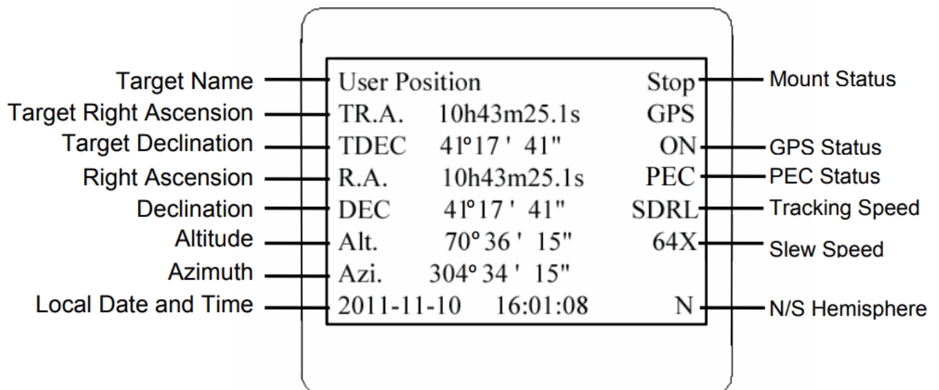
Figure 5. 8407 HC LCD Information Screen
