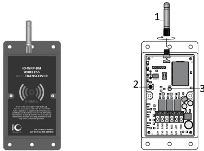
WRP-B BASE TRANSCEIVER ACCESS COVER REMOVED
