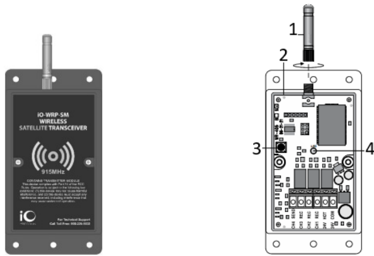
WRP-SATILLITE TRANSCEIVER ACCESS COVER REMOVED
