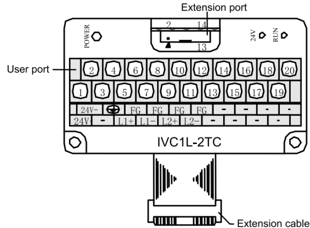
Figure 1-2 IVC1L-2TC ports
