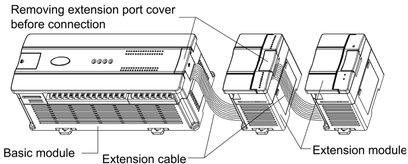
Figure 1-3 Connecting into system
