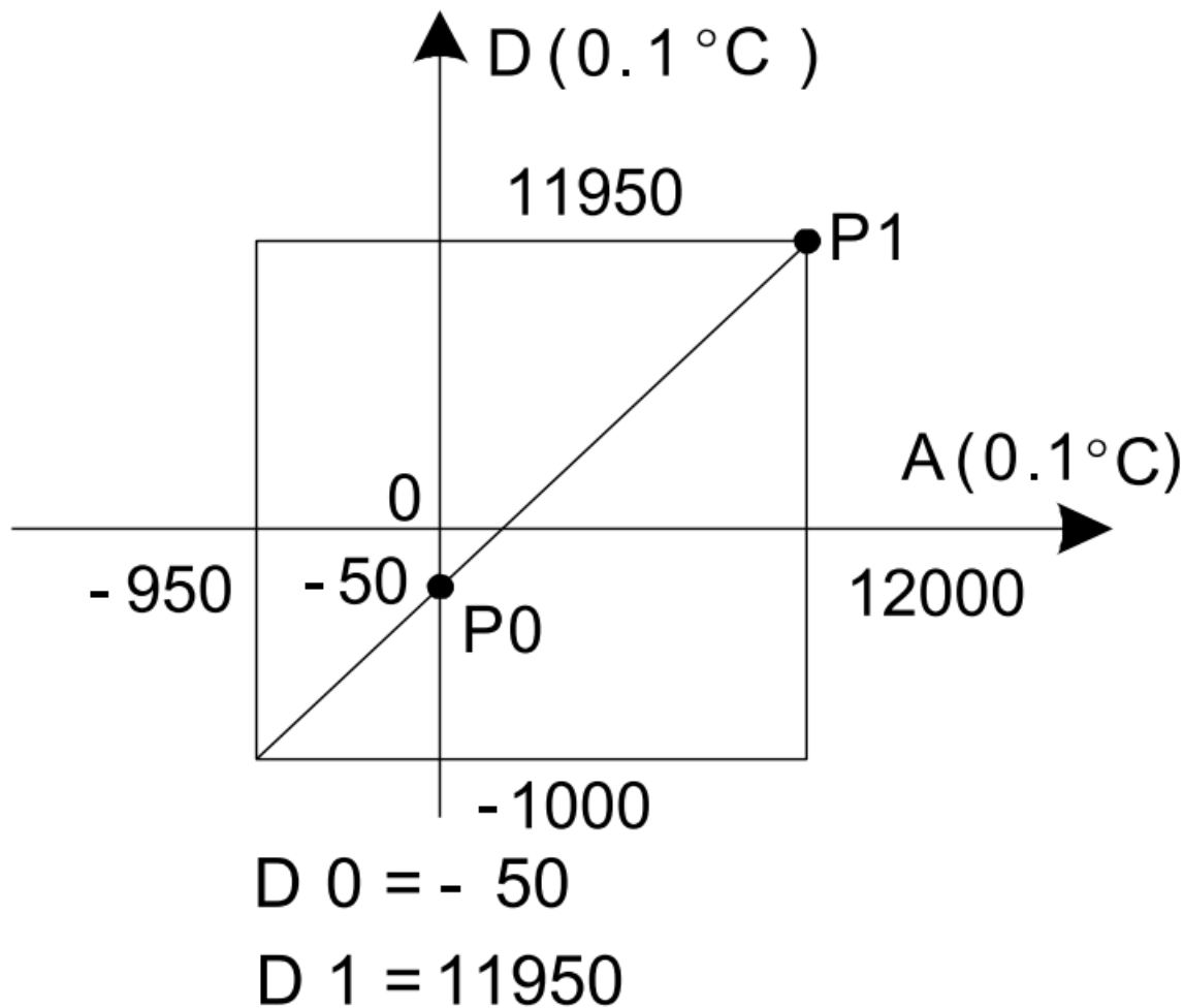
Figure 3-3 Changing characteristic
