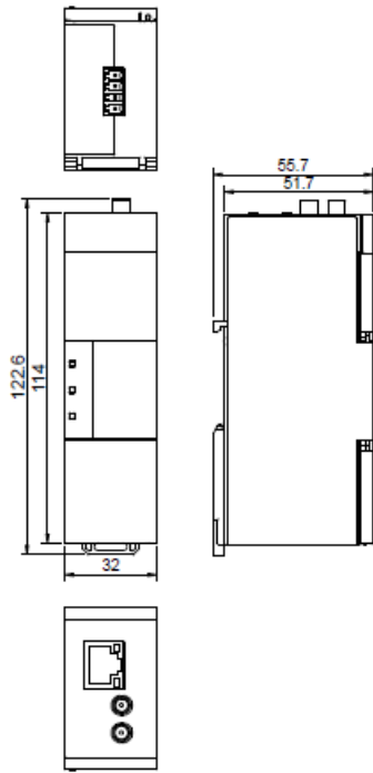
Figure 2-1 ICA413-02 product dimensions
