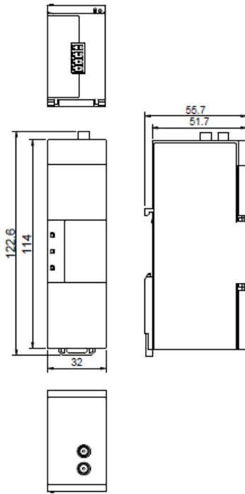
Figure 2-2 ICA400-02 product dimensions
