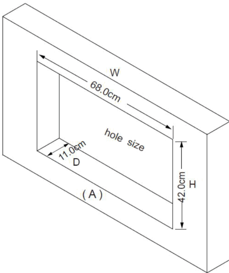
Figure (A) Framing Hole Size
