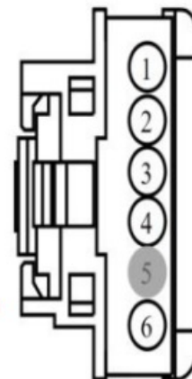
C250 Front of Connector
