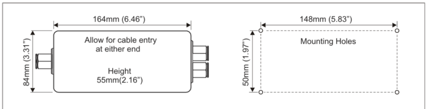
Figure 2.1 Dimensions
