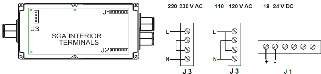
Figure 2.2 Power Connection
