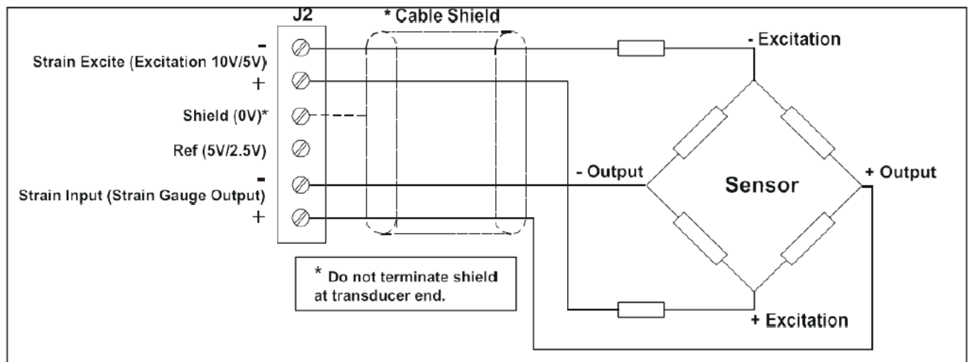
Figure 2.4 Input (Sensor) Connections
