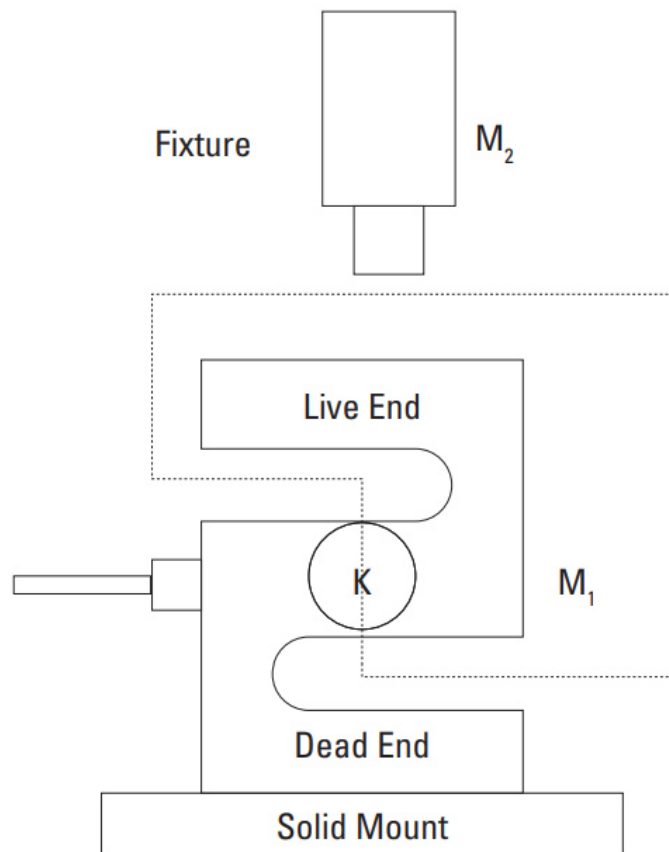
Figure 7. Partitioning of Elements in a Load Cell System
