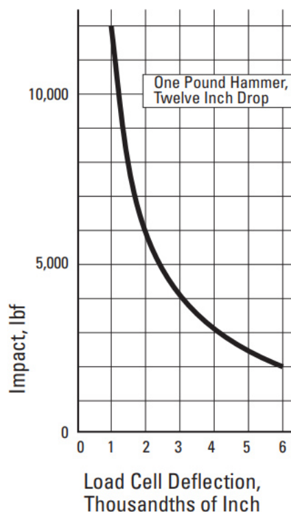
Figure 12. Typical Curve, Impact vs Load Deflection
