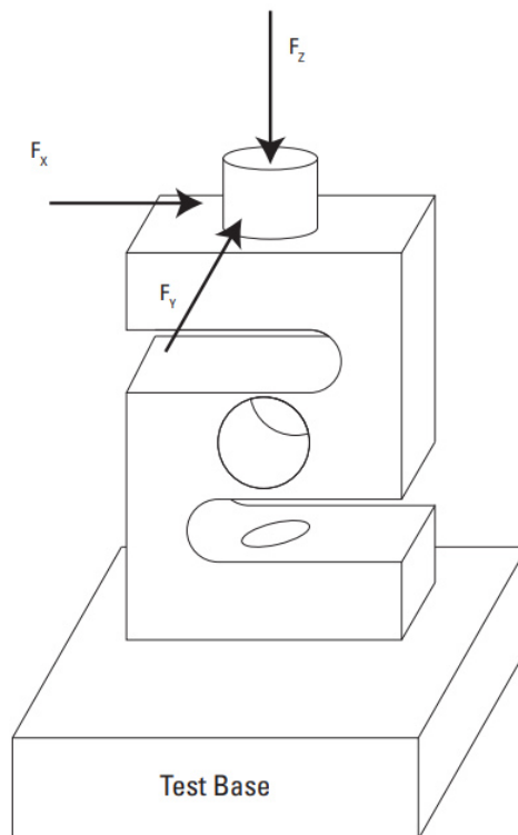
Figure 3. Test Forces Applied to S-Beam Cell.
