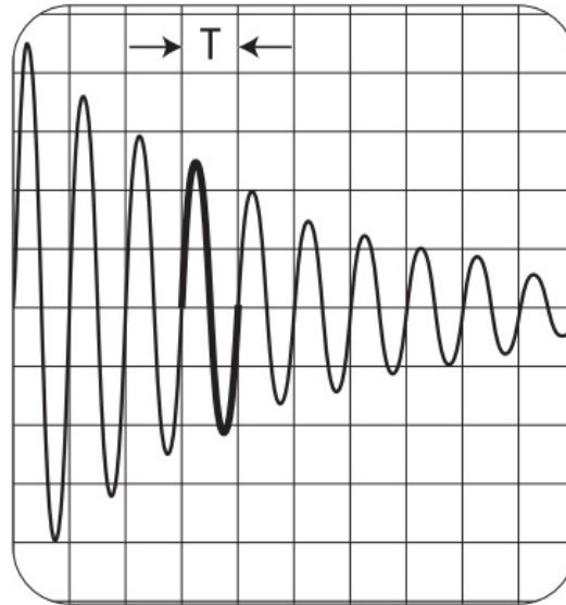
Figure 5. Oscilloscope Trace of Damped Oscillation.
