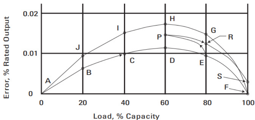
Figure 10. Output Errors with Different Loading Sequences
