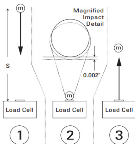
Figure 11. Peak Impact Load
