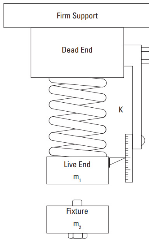
Figure 6. Load Cell Equivalent Elements
