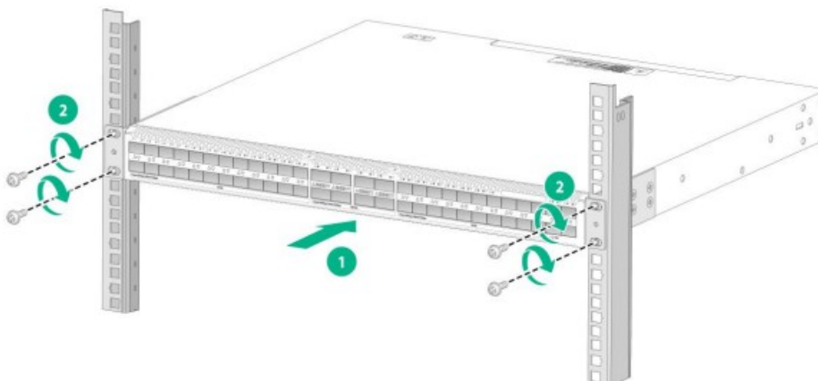
Figure2-4 Mounting the switch in the rack
