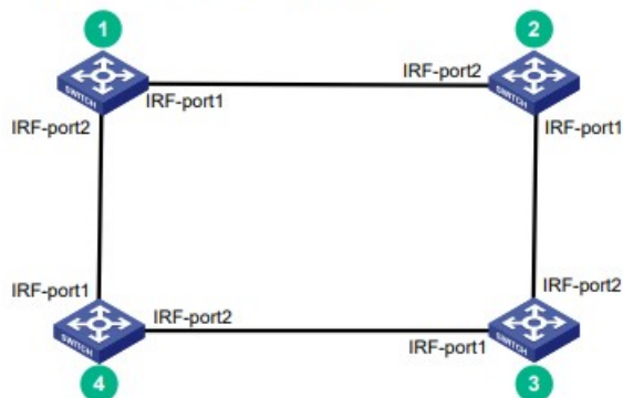
Figure4-5 IRF fabric topology
