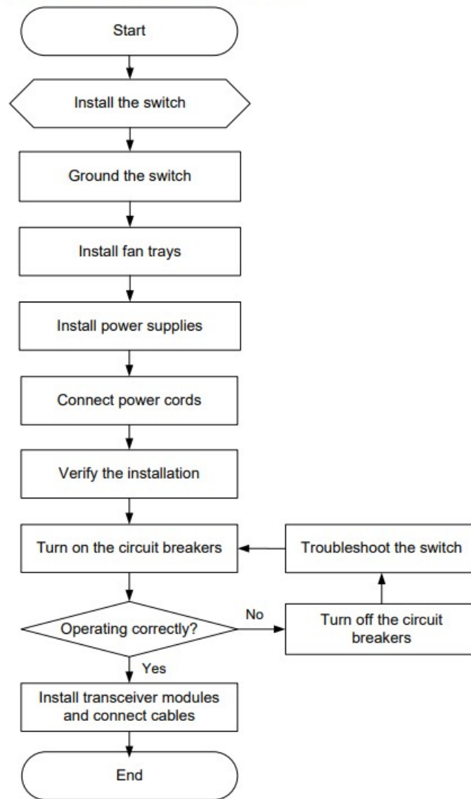
Figure2-1 Hardware installation flow
