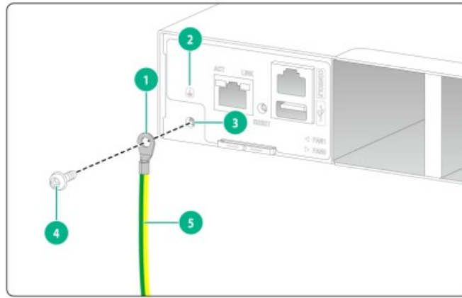
Figure2-5 Connecting the grounding cable to the chassis
