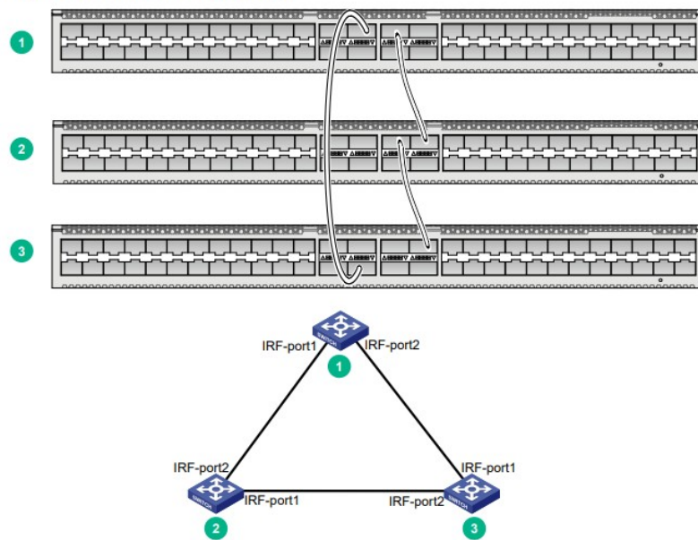
Figure4-3 IRF fabric in ring topology
