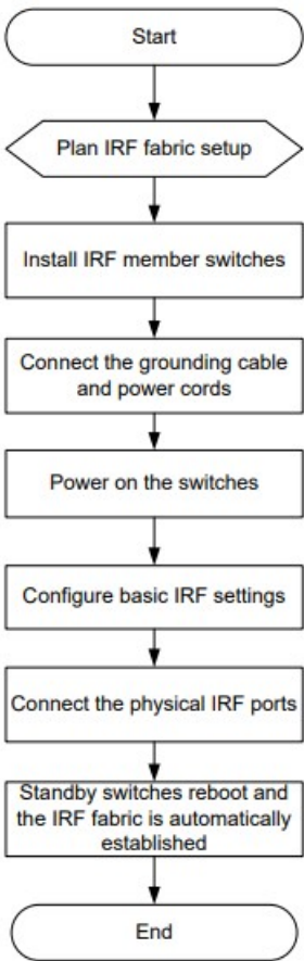
Figure4-1 IRF fabric setup flowchart
