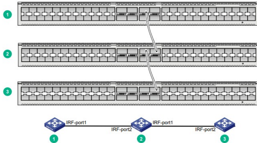
Figure4-2 IRF fabric in daisy chain topology
