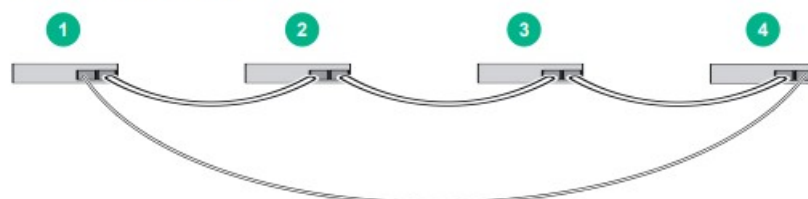
Figure4-6 ToR cabling
