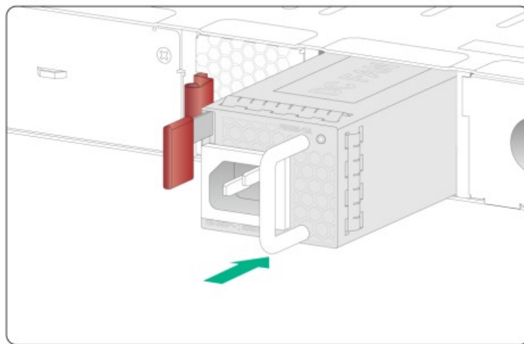
Figure2-12 Installing a power supply
