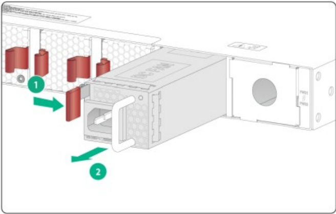
Figure2-13 Removing a power supply
