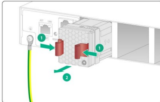
Figure2-8 Removing a fan tray
