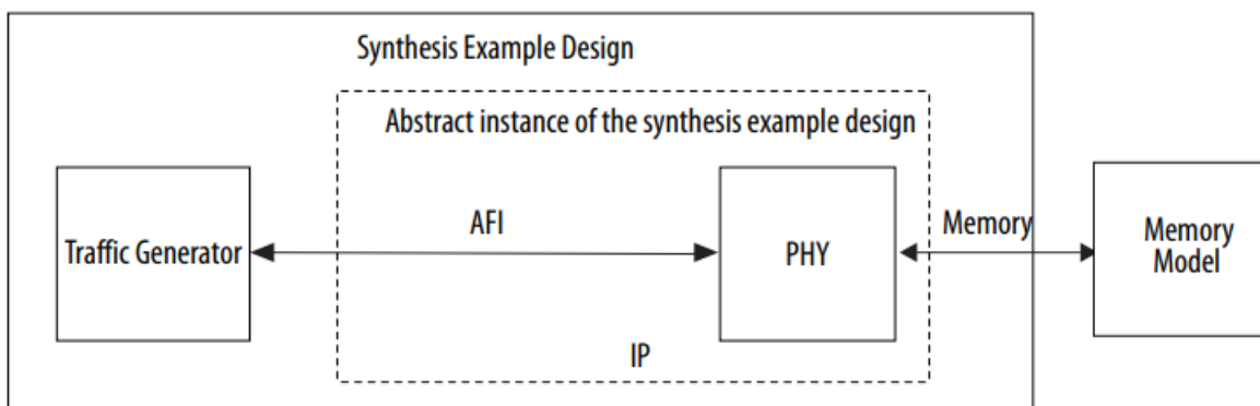
Figure 10. Simulation Example Design for RLDRAM 3 Interfaces
