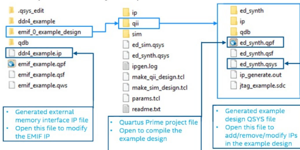
Figure 3. Generated Synthesizable Design Example File Structure
