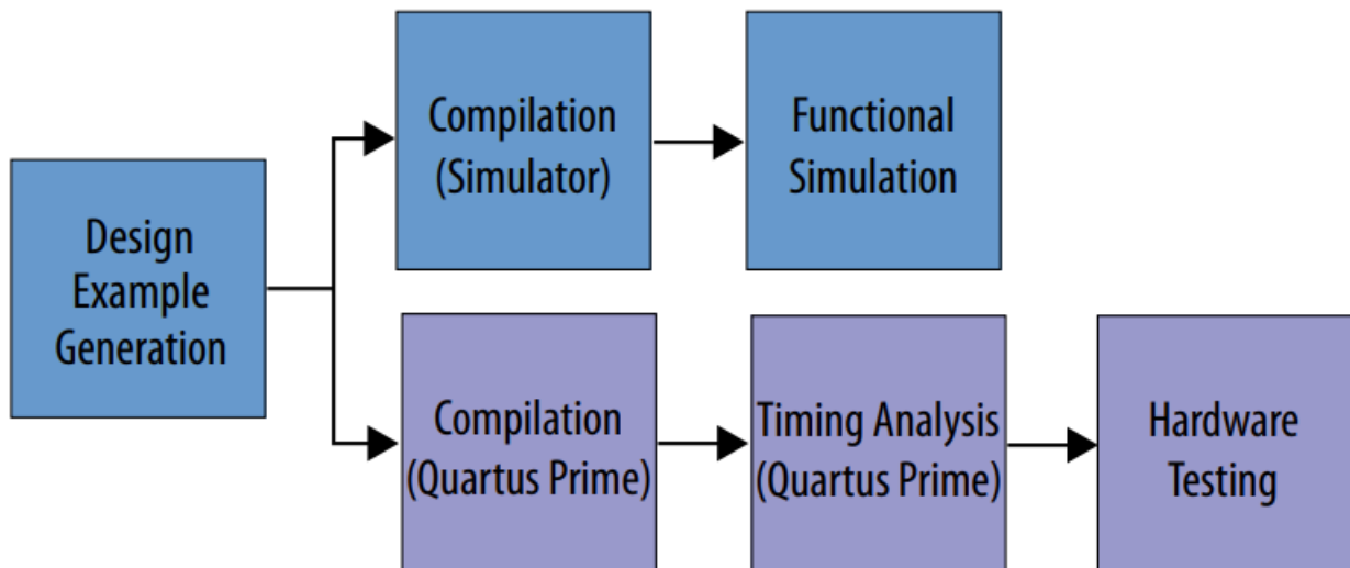
Figure 2. Generating an EMIF Example Design With an Intel Arria 10 Development Kit
