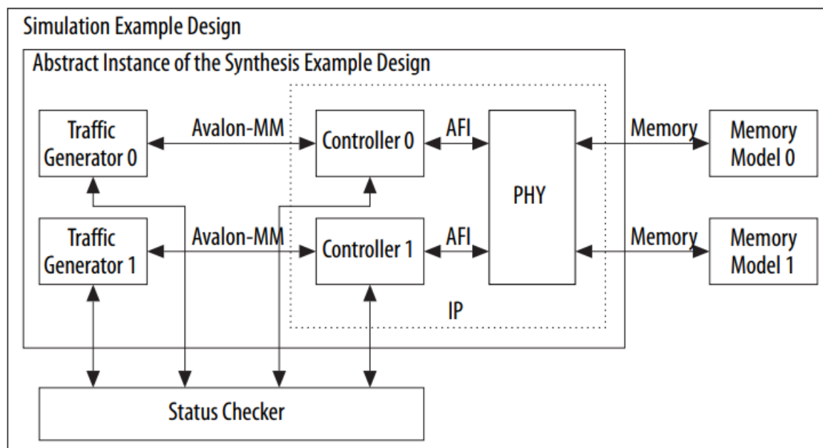
Figure 7. Synthesis Example Design for RLDRAM 3 Interfaces
