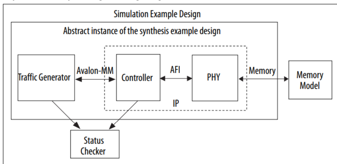
Figure 6. Synthesis Example Design for Ping Pong PHY
