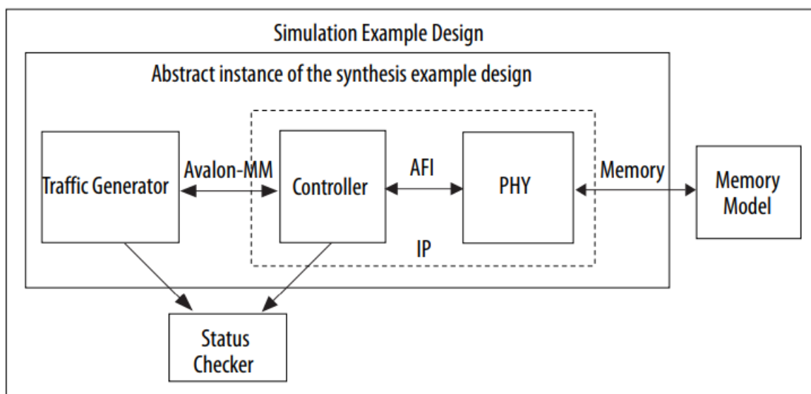
Figure 8. Simulation Example Design
