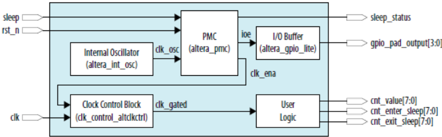
Input and Output Ports of the Power Management Controller Reference Design
