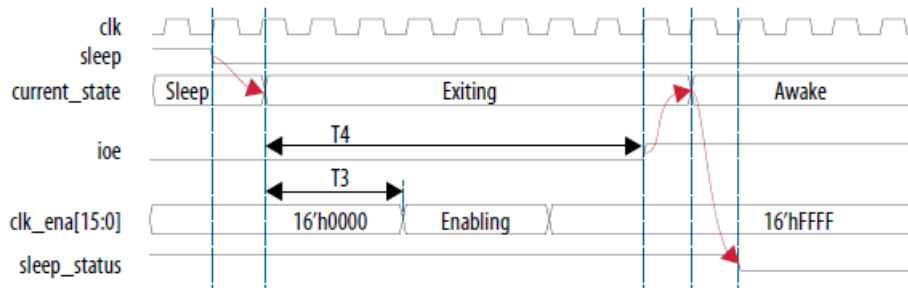
Figure 11. Exiting Sleep Mode Timing Diagram
