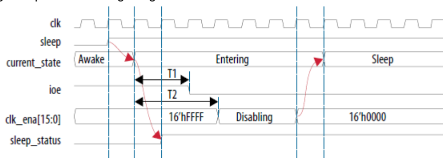
Figure 10. Entering Sleep Mode Timing Diagram
