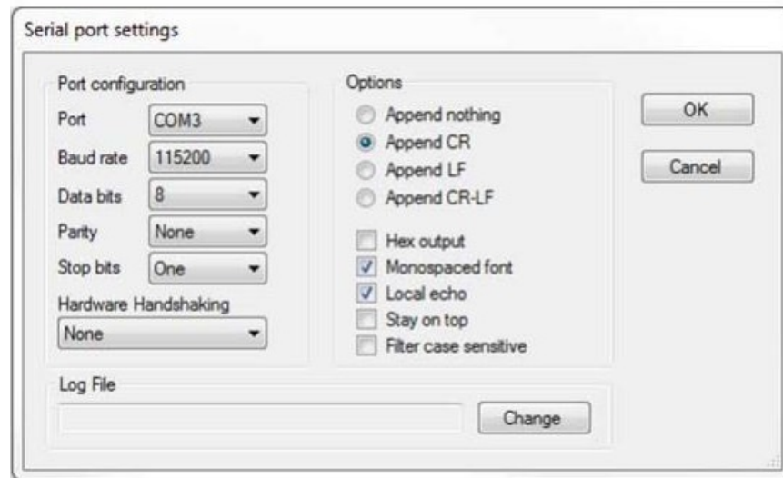
Figure 4: UART Serial Port Settings Screen Capture
