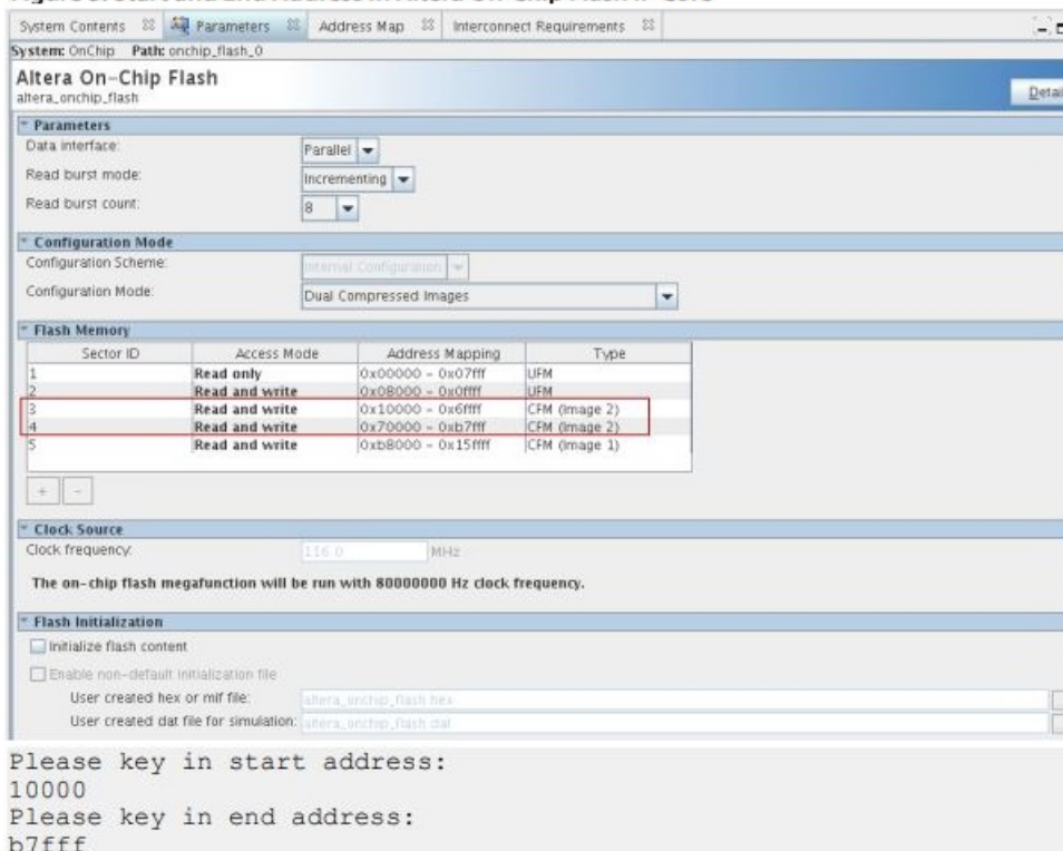
Figure 5: Start and End Address in Altera On-Chip Flash IP Core
