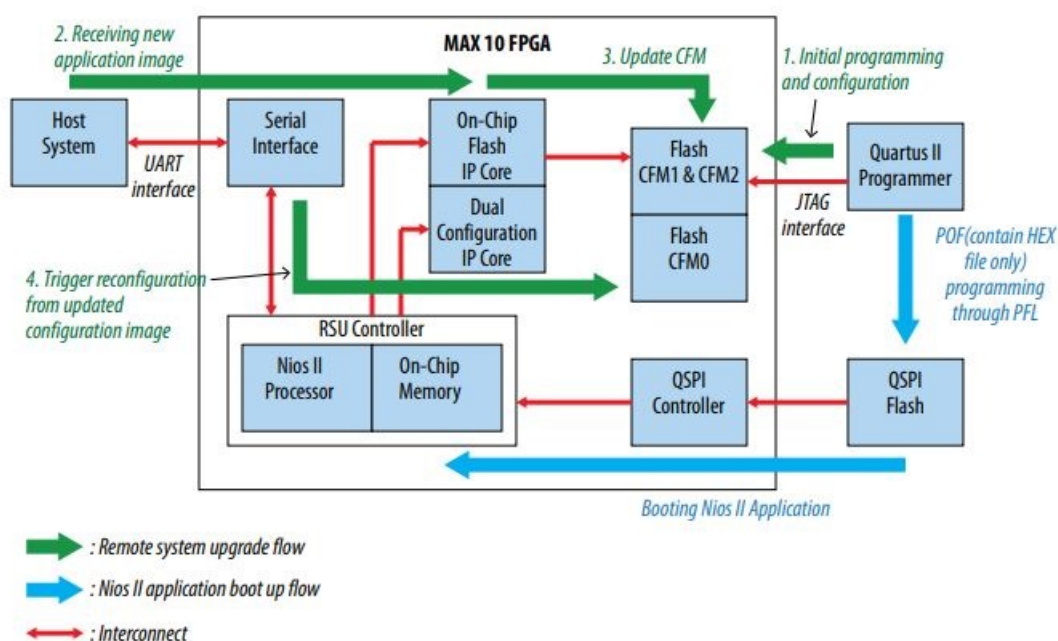
Figure 1: Reference Design Block Diagram
