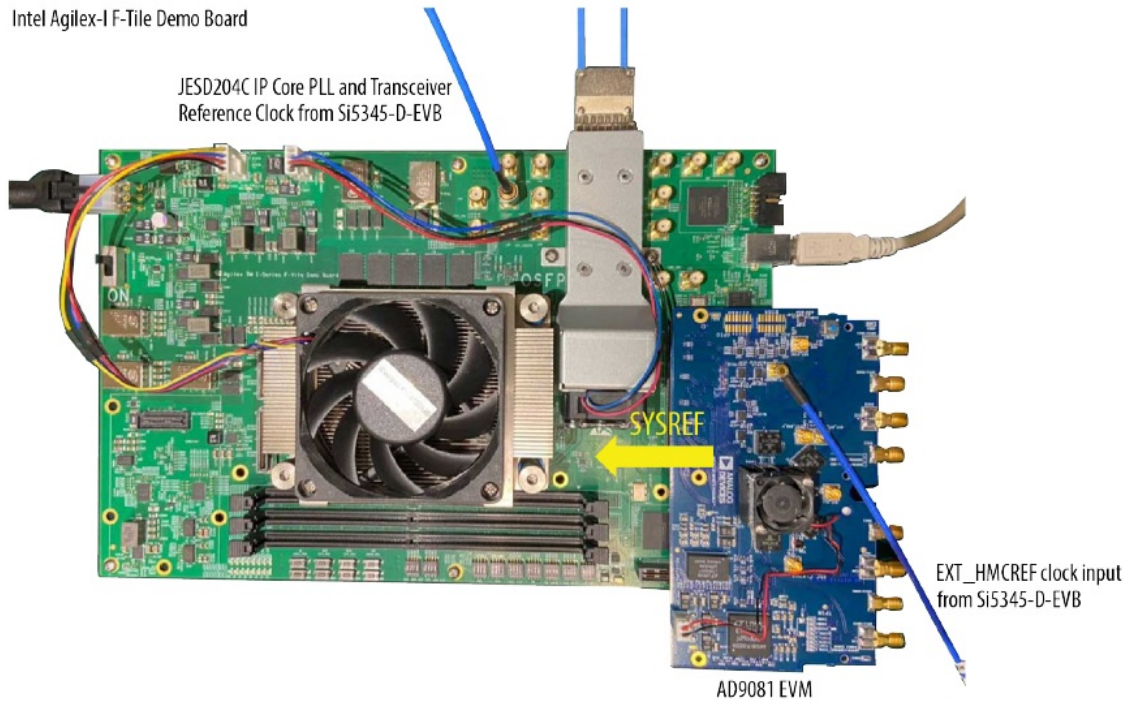
Figure 1. Hardware Setup
