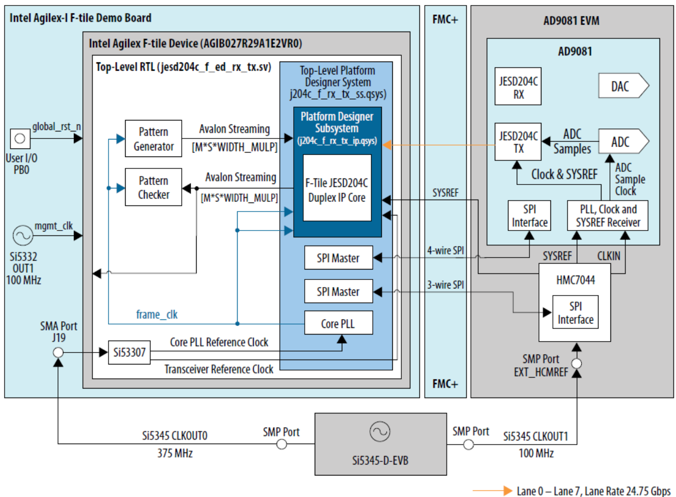
Figure 2. System Diagram
