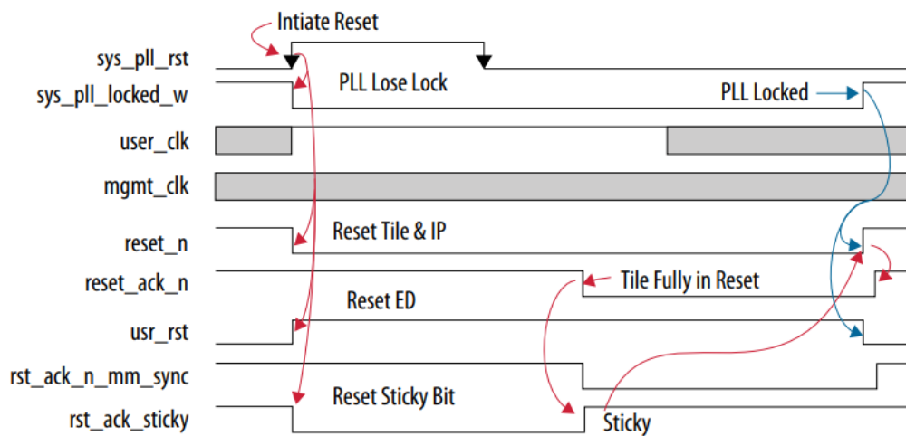
Figure 8. Reset Sequence in PAM4 Mode
