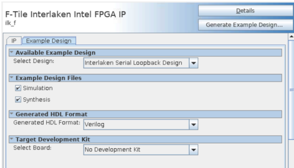
Figure 4. Example Design Tab
