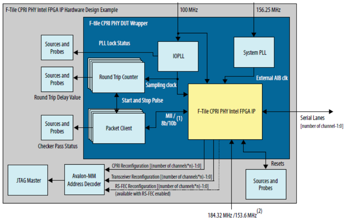
Figure 8. Hardware Design Example Block Diagram
