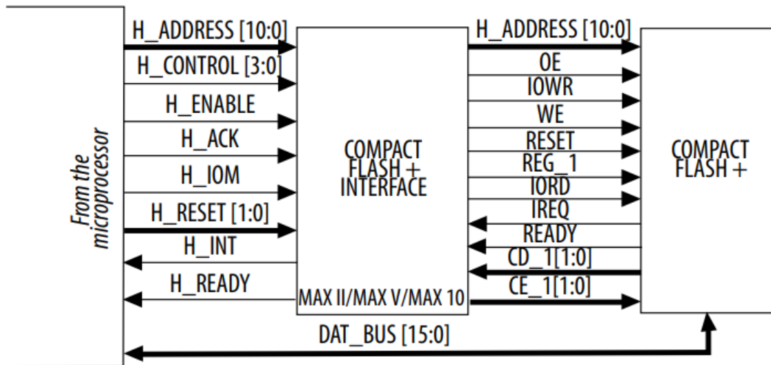
Figure 1: The Different Interfacing Signals of the CF+ Interface and the CF+ Device
