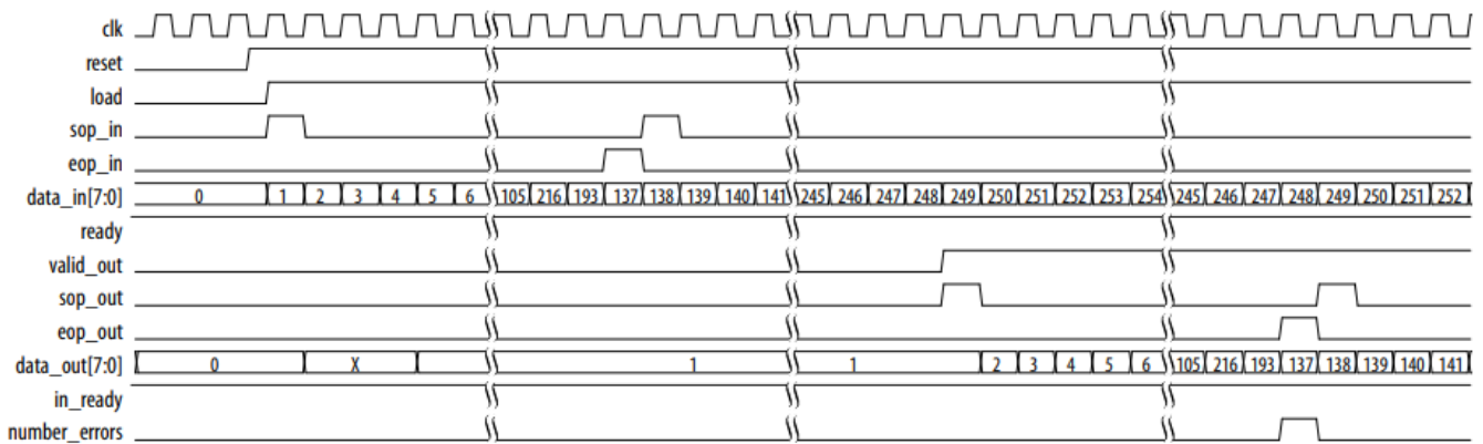
Figure 8. Decoder Timing
