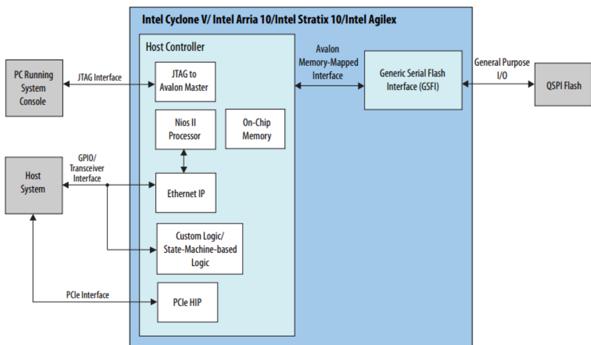
Figure 5. Accessing QSPI Flash
