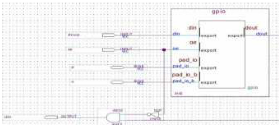
Input and Output Ports Connection Example for Intel Stratix 10 Devices
