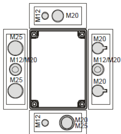
Fig. 4 Housing knockouts
