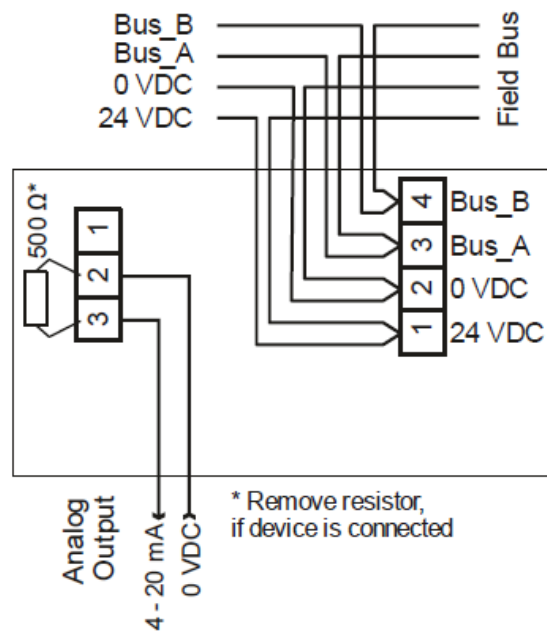
Fig 3: Electrical connection with option analog output
