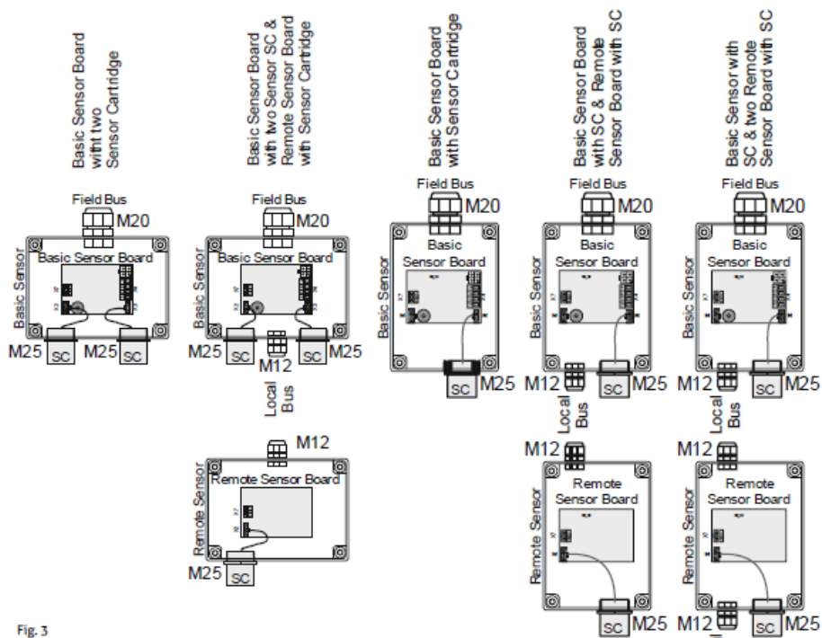
Fig. 3 Mounting possibilities
