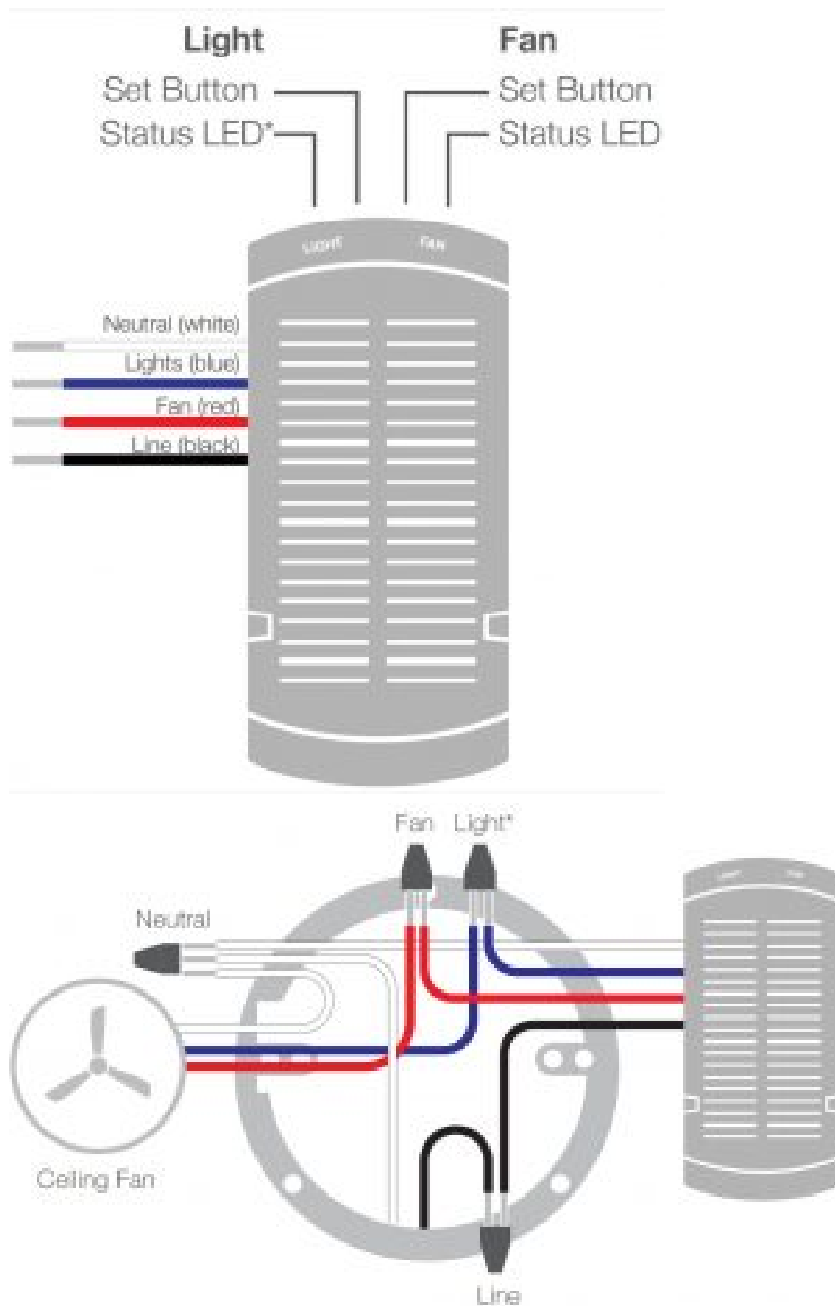
(Wiring Diagram)
