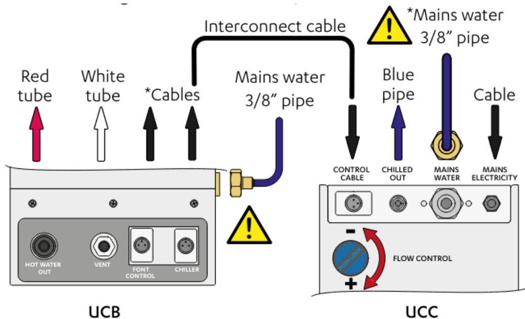
I2CB10 Boiling models (top view)
