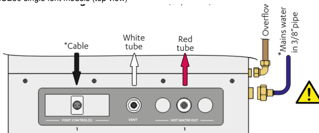
I2CB20 - I2CB50 single font models (top view)
