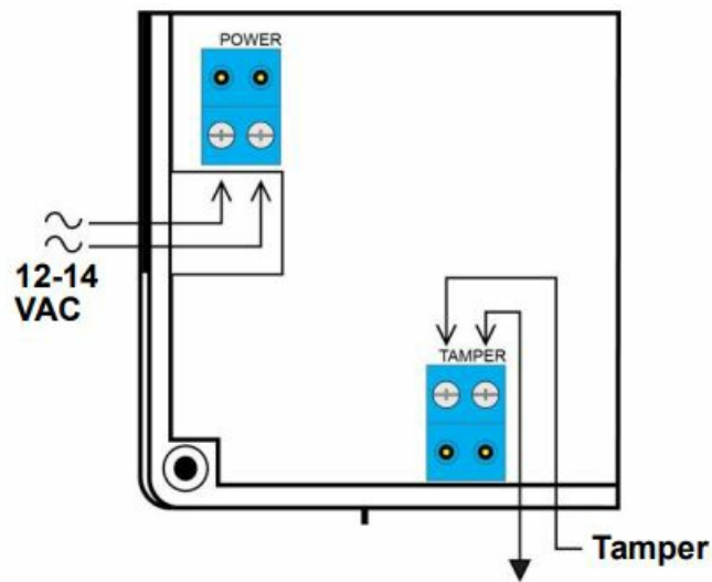
Figure 4 Power and tamper wiring
