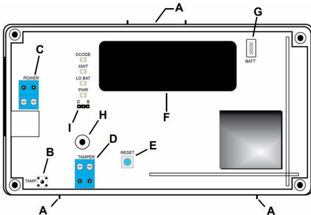
Figure 3 High power repeater internal components
