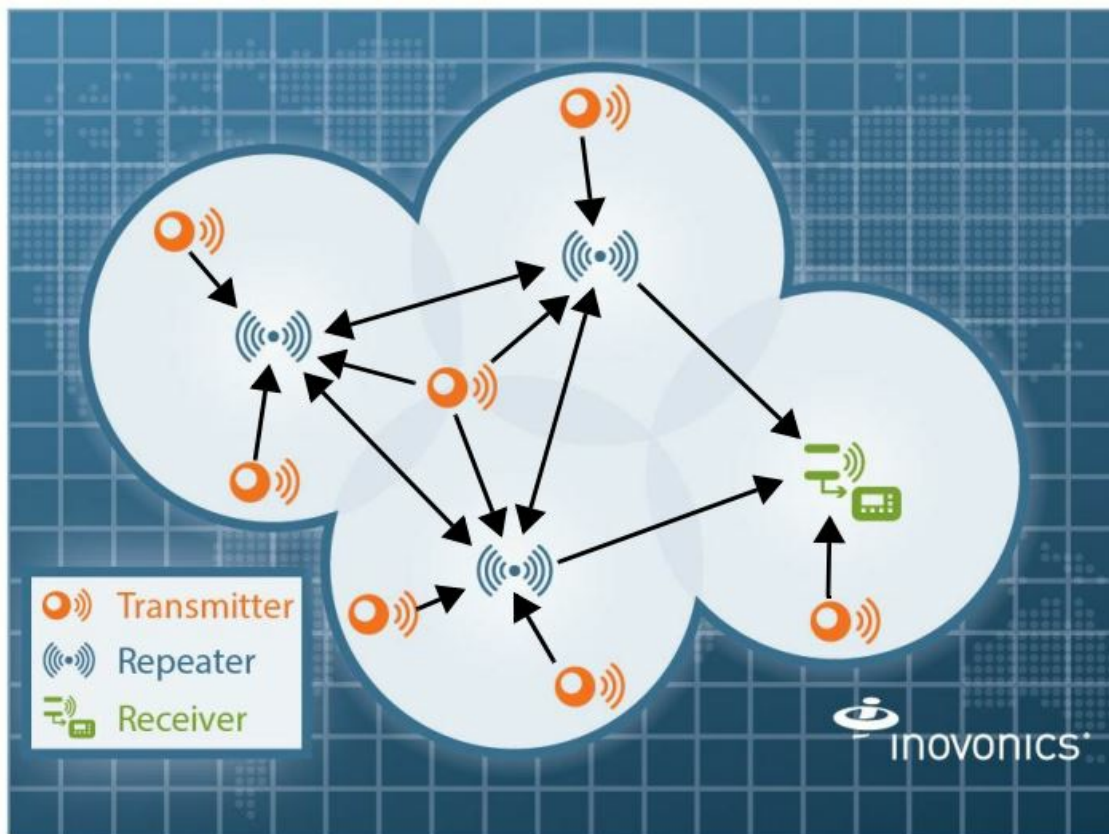
Figure 1 Sample EchoStream system
