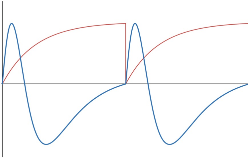
Figure 2: “Bent” phasor and resulting distorted waveform
