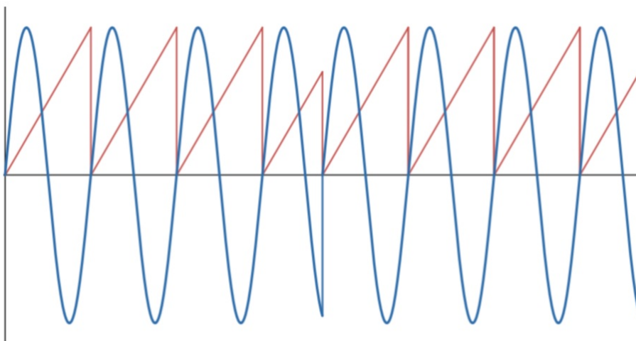
Sync - two fundamental periods of 0° Output demonstrating “hard sync” behavior
